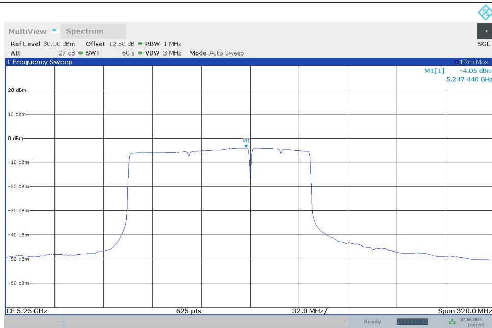
11BE160MIMO_Ant1_5250_996+484+242_OFDMA_1
