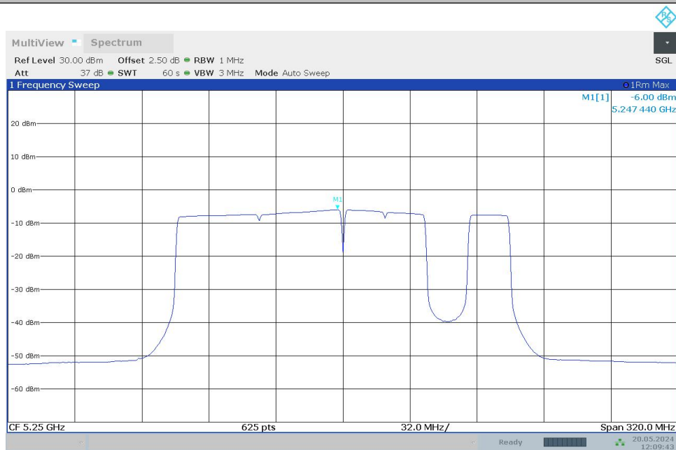
11BE160MIMO_Ant1_5250_996+484+242_OFDMA_7
