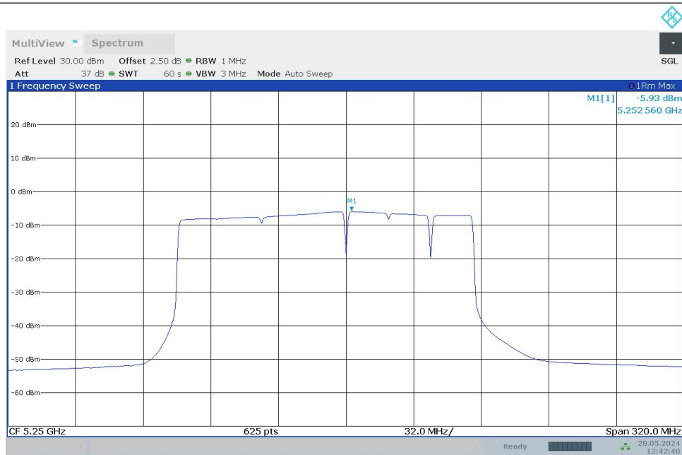
11BE160MIMO_Ant1_5250_996+484_OFDMA_1
