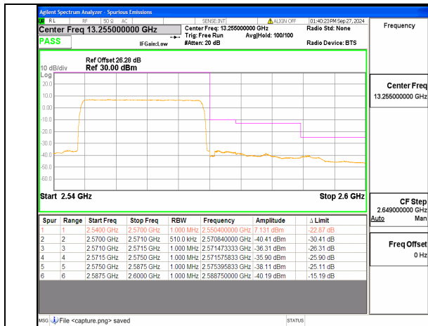
n7 25M DFT-s-OFDM QPSK Outer_Full High
