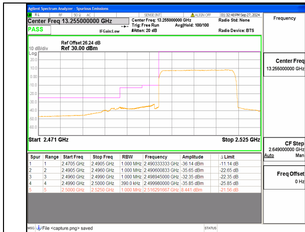
n7 20M DFT-s-OFDM QPSK Outer_Full Low
