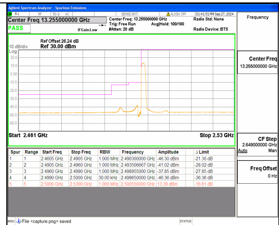
n7 30M DFT-s-OFDM BPSK Edge_1RB_Left Low
