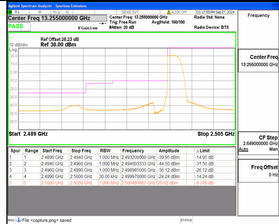
n7 5M DFT-s-OFDM QPSK Edge_1RB_Left Low
