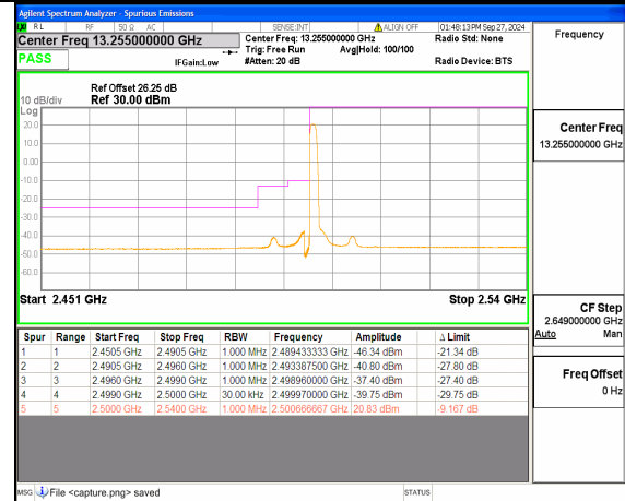
n7 40M DFT-s-OFDM QPSK Edge_1RB_Left Low
