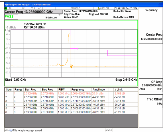
n7 40M DFT-s-OFDM BPSK Edge_1RB_Right High
