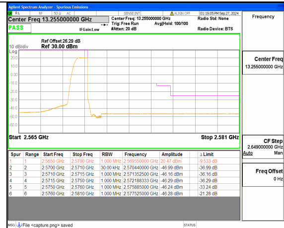
n7 5M DFT-s-OFDM BPSK Edge_1RB_Right High
