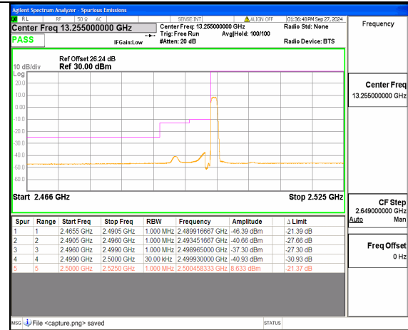
n7 25M DFT-s-OFDM BPSK Edge_1RB_Left Low
