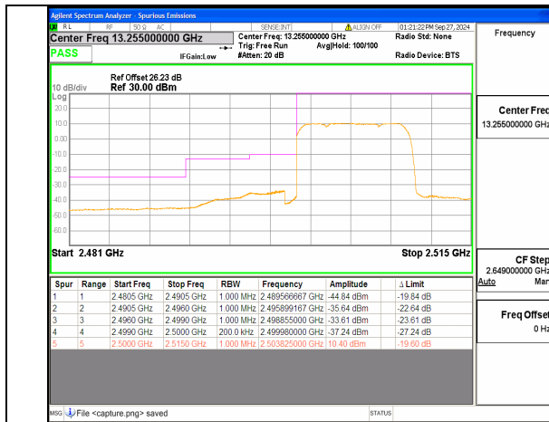
n7 10M DFT-s-OFDM BPSK Outer_Full Low
