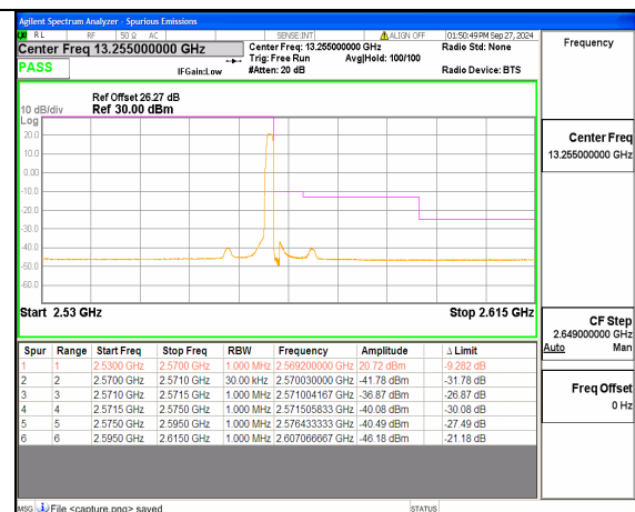
n7 40M DFT-s-OFDM QPSK Edge_1RB_Right High
