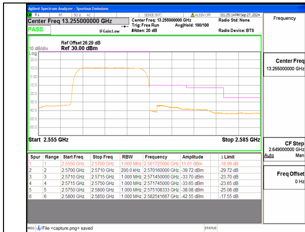
n7 10M DFT-s-OFDM QPSK Outer_Full High
