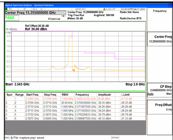
n7 25M DFT-s-OFDM QPSK Edge_1RB_Right High
