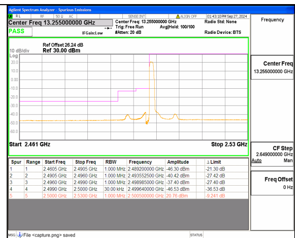
n7 30M DFT-s-OFDM QPSK Edge_1RB_Left Low
