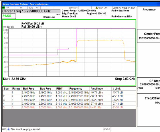
n7 25M DFT-s-OFDM BPSK Outer_Full Low
