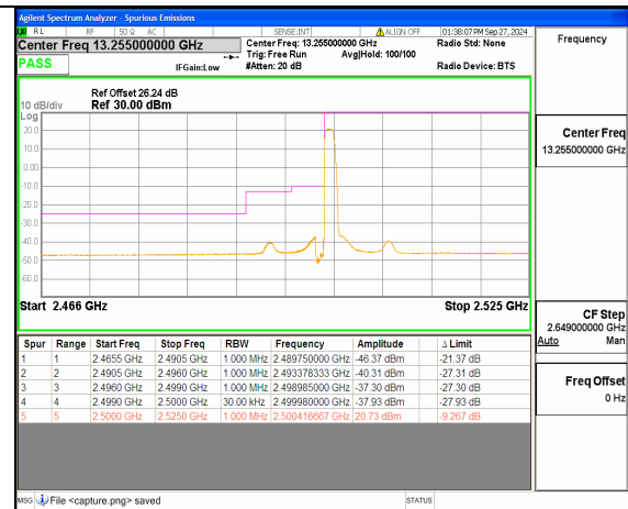
n7 25M DFT-s-OFDM QPSK Edge_1RB_Left Low
