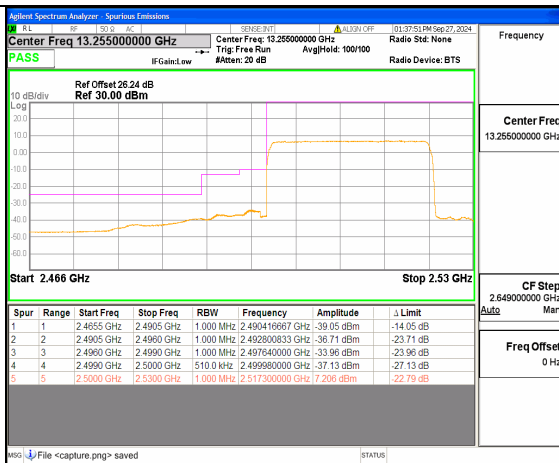
n7 25M DFT-s-OFDM QPSK Outer_Full Low
