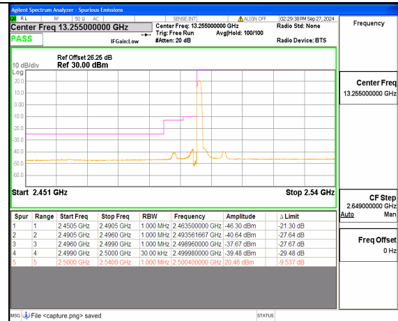
n7 40M DFT-s-OFDM BPSK Edge_1RB_Left Low
