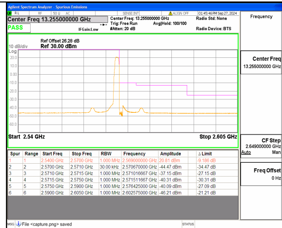
n7 30M DFT-s-OFDM QPSK Edge_1RB_Right High
