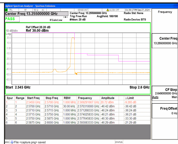
n7 25M DFT-s-OFDM BPSK Edge_1RB_Right High
