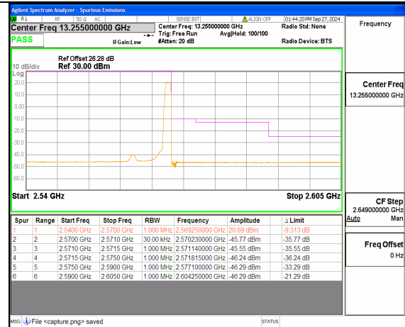
n7 30M DFT-s-OFDM BPSK Edge_1RB_Right High
