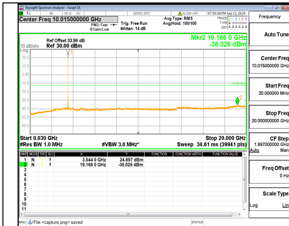
n78(3450-3550MHz) (30MHz-20GHz) 90M DFT-s-OFDM QPSK Inner_1RB_Right Mid
