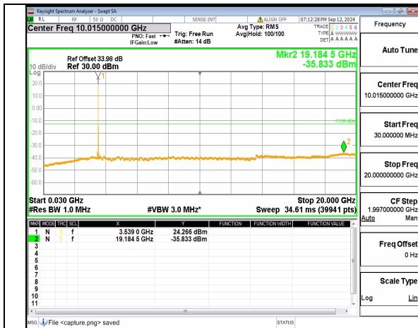
n78(3450-3550MHz) (30MHz-20GHz) 80M DFT-s-OFDM QPSK Inner_1RB_Right Mid
