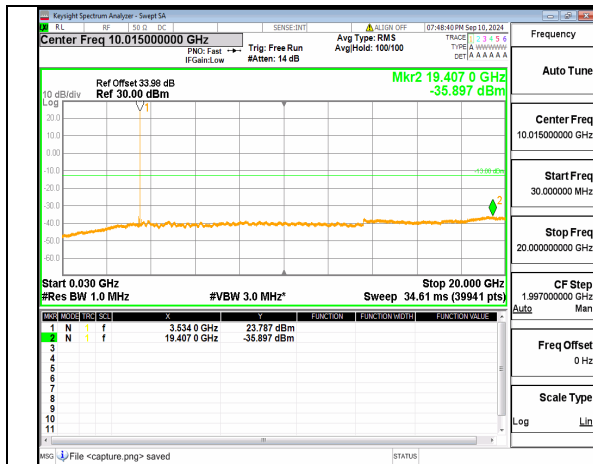
n77(3450-3550MHz) (30MHz-20GHz) 70M DFT-s-OFDM BPSK Inner_1RB_Right Mid
