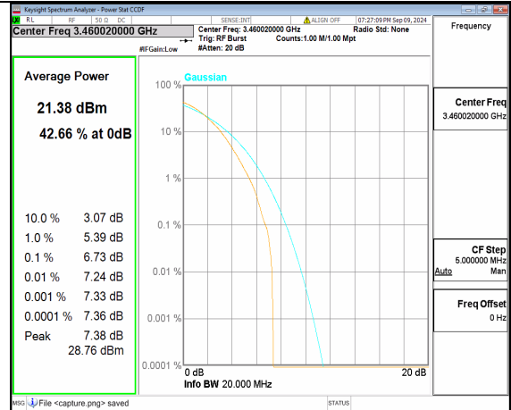
n78(3450-3550MHz) 20M DFT-s-OFDM 256QAM Outer_Full Low
