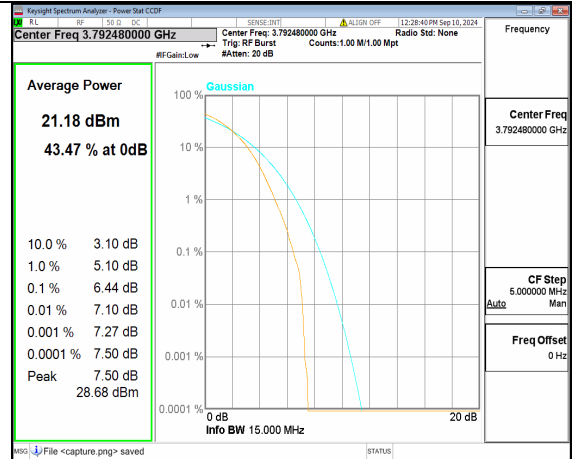
n78(3700-3800MHz) 15M DFT-s-OFDM 256QAM Outer_Full High
