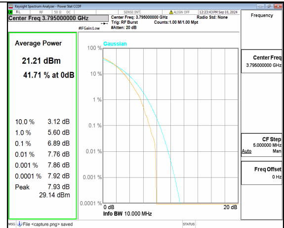
n78(3700-3800MHz) 10M DFT-s-OFDM 256QAM Outer_Full High
