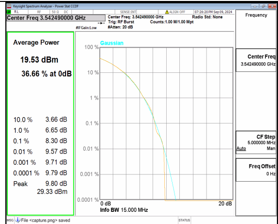
n78(3450-3550MHz) 15M CP-OFDM 256QAM Outer_Full High
