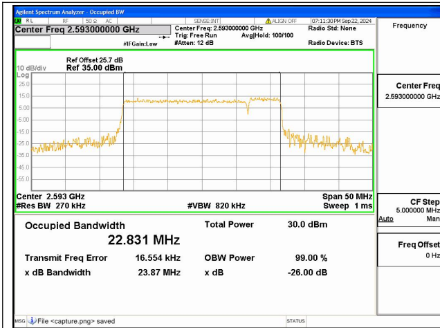
41C / 20+5MHz / 64QAM/ Mid CH
