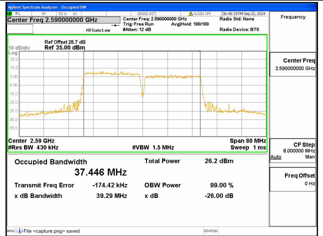
38C / 20+20MHz / 256QAM/ Low CH
