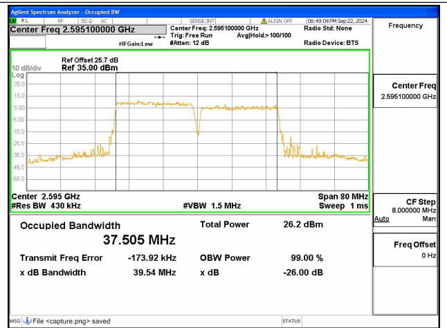
38C / 20+20MHz / 256QAM/ Mid CH
