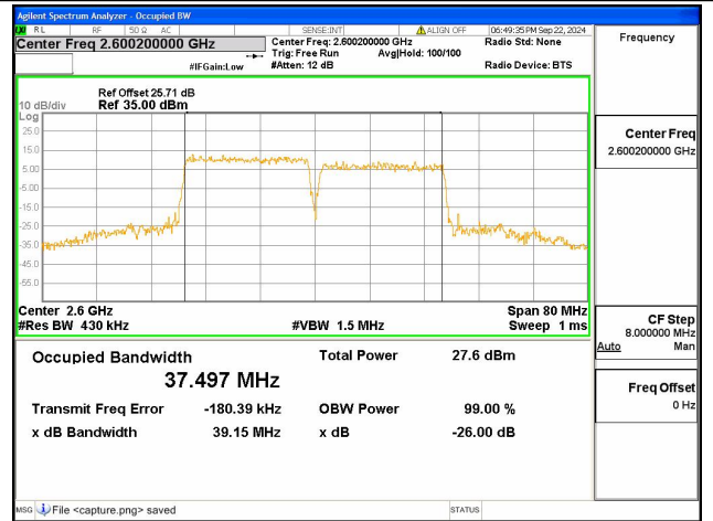
38C / 20+20MHz / 16QAM/ High CH
