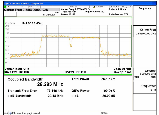
38C / 15+15MHz / 256QAM/ Low CH
