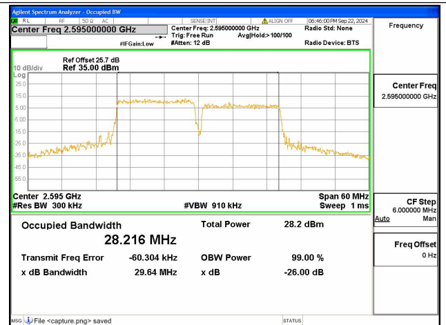
38C / 15+15MHz / 16QAM/ Mid CH
