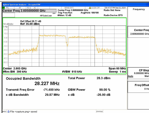
38C / 15+15MHz / 64QAM/ High CH
