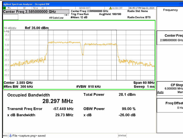
38C / 15+15MHz / 64QAM/ Low CH
