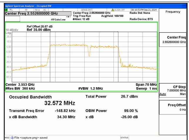
7C / 20+15MHz / 256QAM/ High CH
