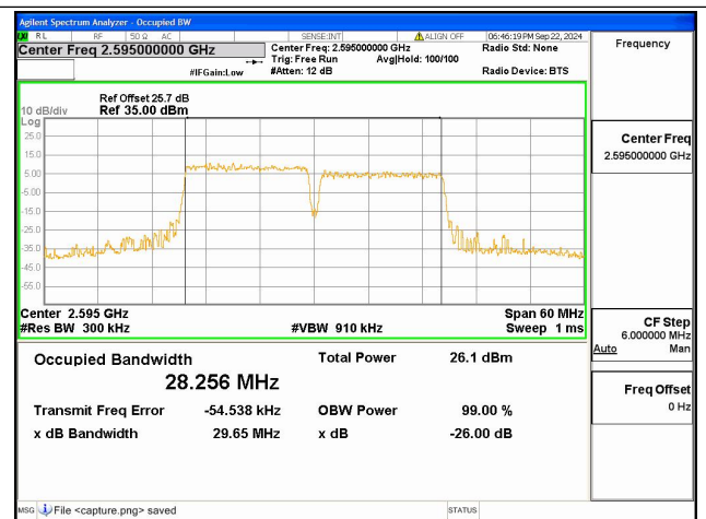
38C / 15+15MHz / 256QAM/ Mid CH
