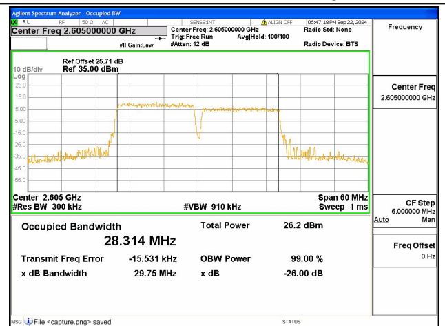
38C / 15+15MHz / 256QAM/ High CH
