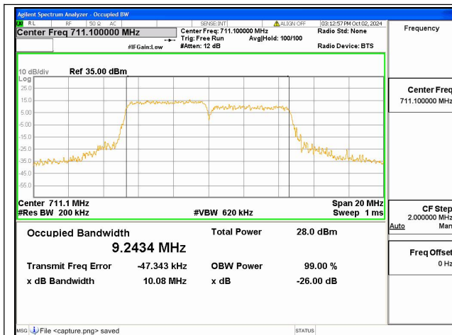
12B / 5+5MHz / 64QAM/ High CH
