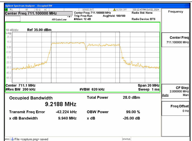
12B / 5+5MHz / 16QAM/ High CH
