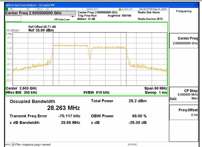
38C / 15+15MHz / 16QAM/ High CH
