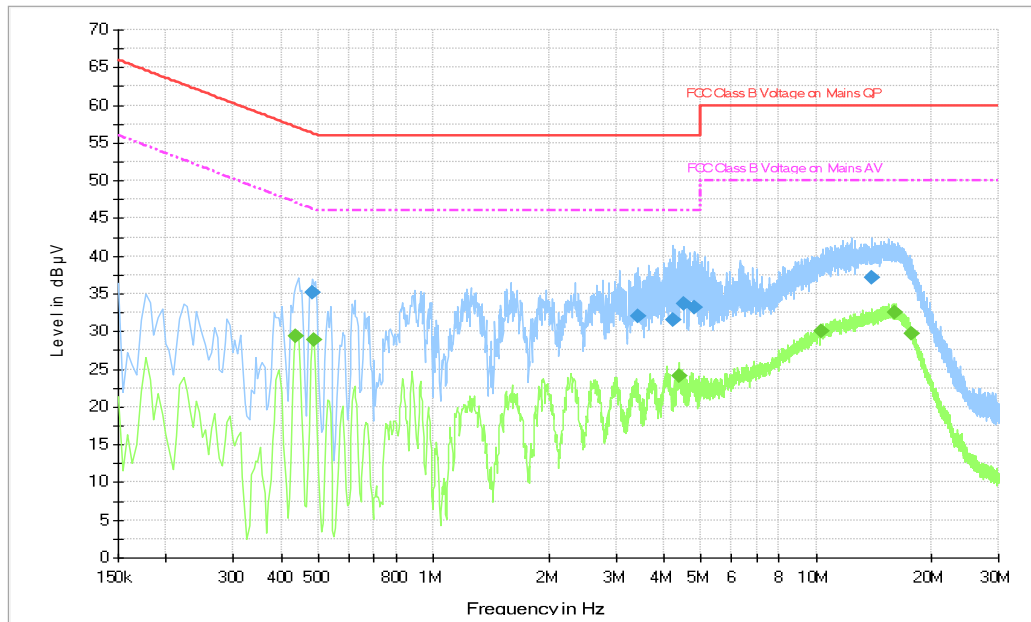
Fig.B.9.3 AC Powerline Conducted Emission- bluetooth(Charger WC030B51HK)
