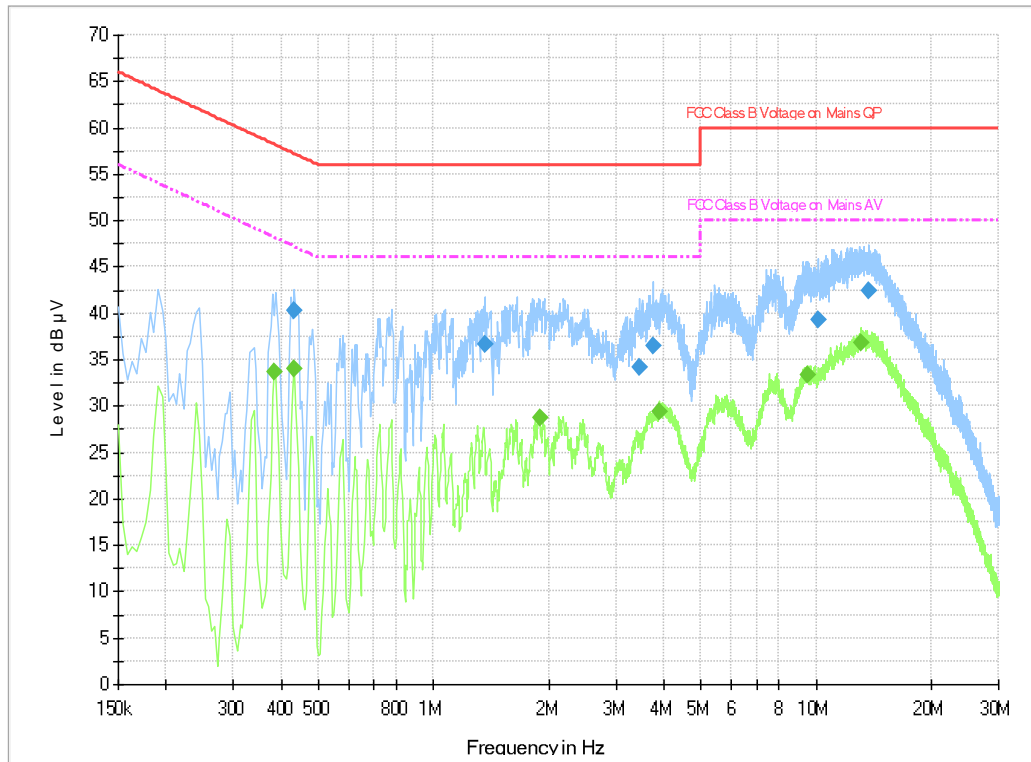
Fig.B.9.2 AC Powerline Conducted Emission-Idle(Charger WC0506A51JH)
