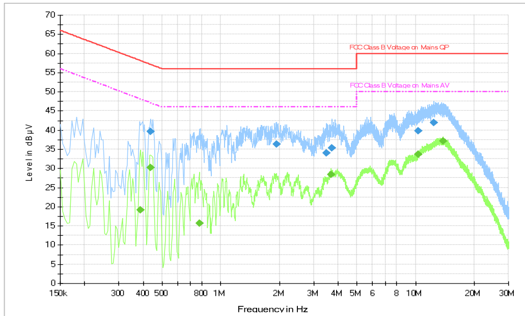
Fig.B.9.1 AC Powerline Conducted Emission- bluetooth(Charger WC0506A51JH)
