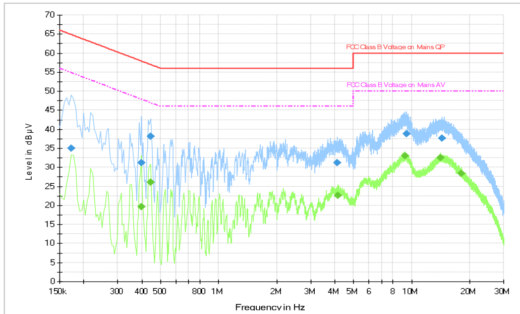
Fig.B.9.4 AC Powerline Conducted Emission(Charger WC0506A51GB)
