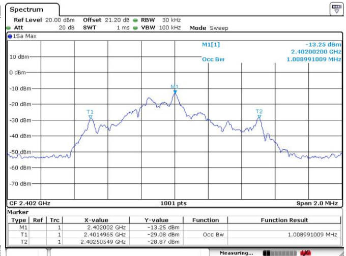
99% Bandwidth Plot on 2402MHz
