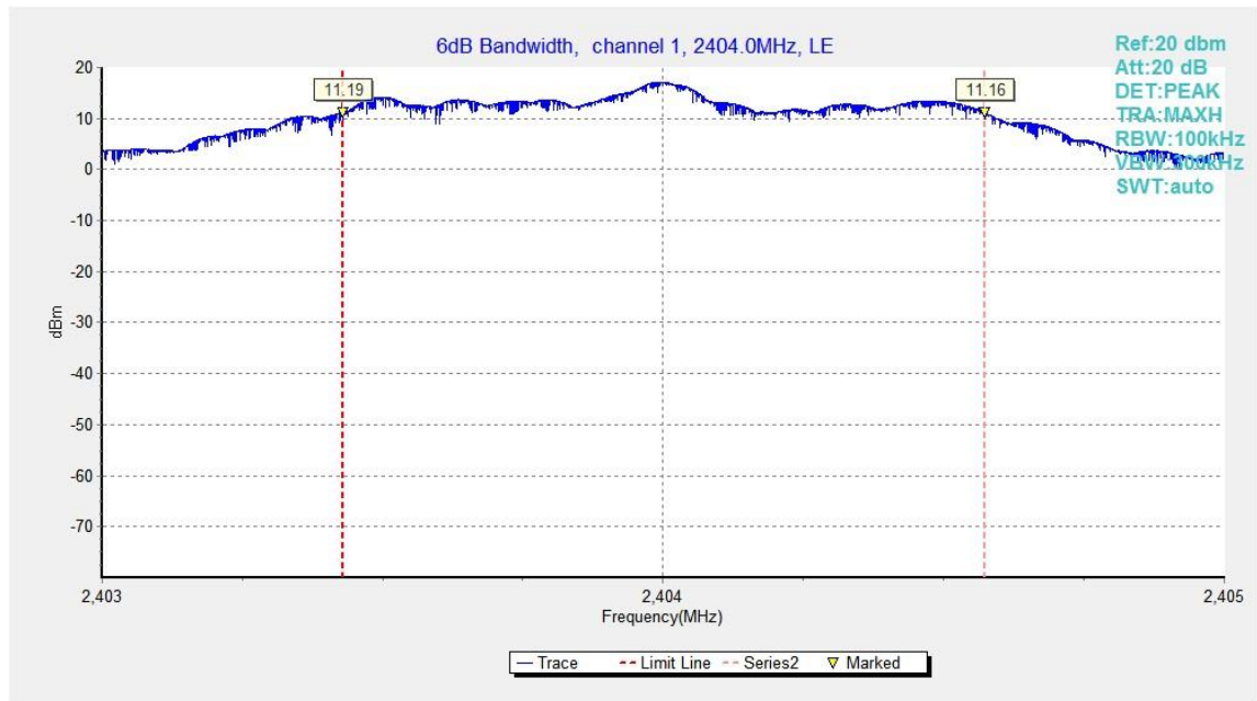
Fig.22. 6dB Bandwidth: GFSK, 2404 MHz
