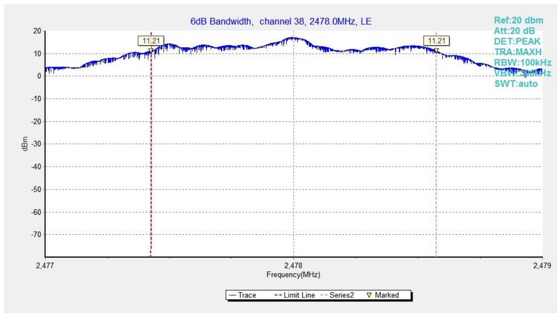
Fig.24. 6dB Bandwidth: GFSK, 2478 MHz
