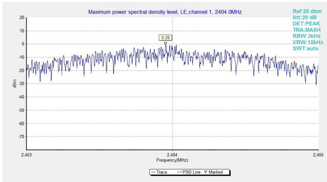
Fig.25. Maximum Power Spectral Density Level Function: GFSK, 2404 MHz
