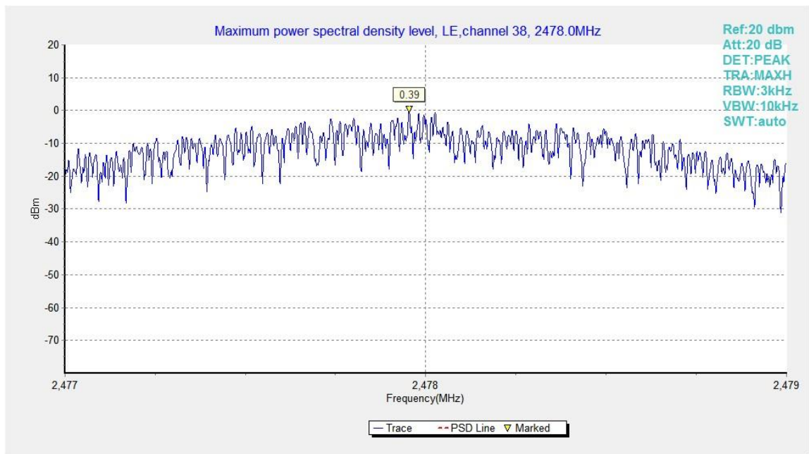
Fig.27. Maximum Power Spectral Density Level Function: GFSK, 2478 MHz
