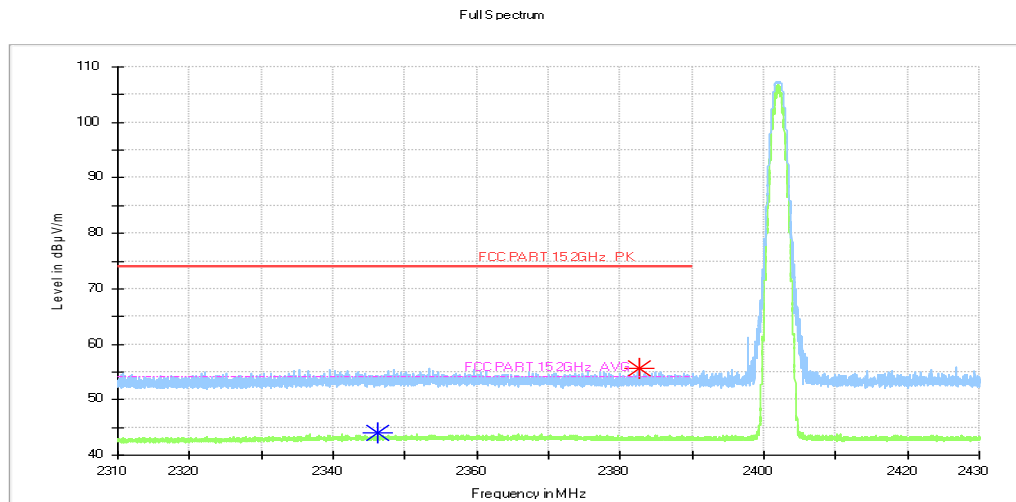
Fig.18. Frequency Band Edges: GFSK, LE 1M 2402 MHz, 2.31 GHz – 2.43GHz
