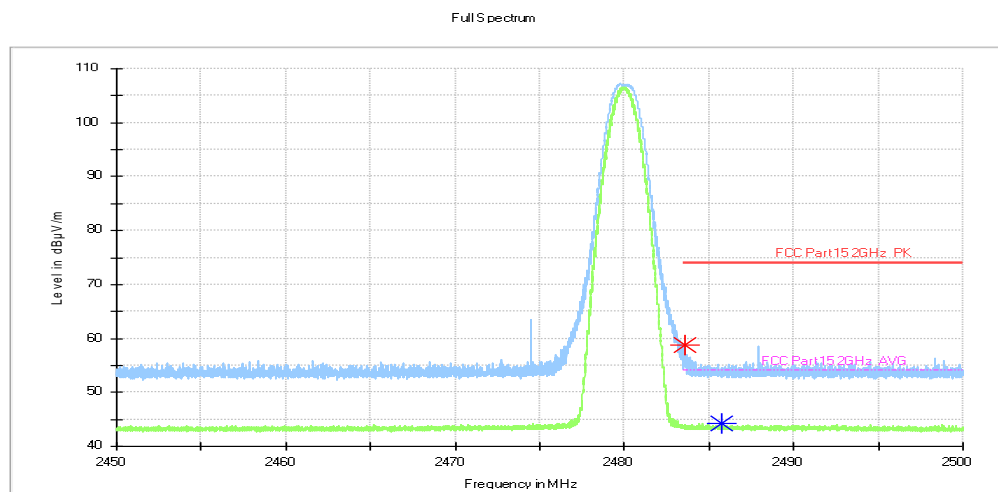
Fig.19. Frequency Band Edges: GFSK, LE 1M 2480 MHz, 2.45 GHz - 2.50GHz
