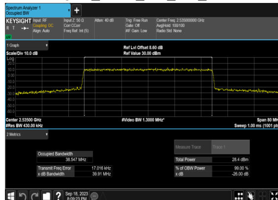
N7(40M)_CP-OFDM_16 QAM_Outer_Full_Mid_CH
