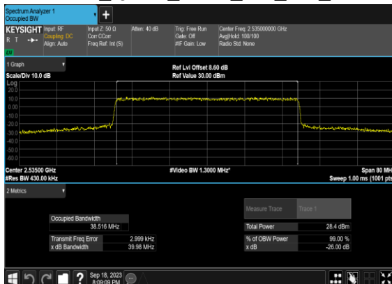
N7(40M)_CP- OFDM_QPSK_Outer_Full_Mid_CH
