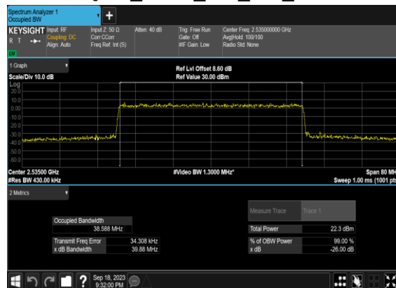
N7(40M)_CP-OFDM_256 QAM_Outer_Full_Mid_CH
