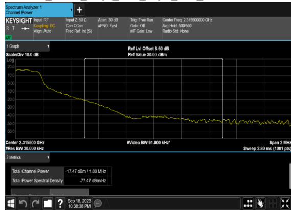
N30(10M)_DFT-s- OFDM_BPSK_Edge_1RB_Right_Low_CH_CHP_PASS
