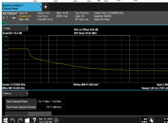
N30(5M)_DFT-s- OFDM_BPSK_Outer_Full_High_CH_CHP_PASS
