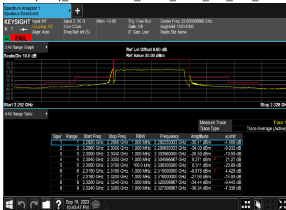
N30(10M)_DFT-s-OFDM_BPSK_Outer_Full_Low_CH
