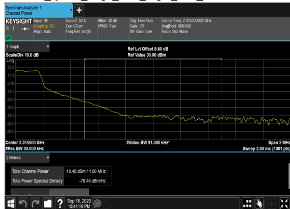
N30(10M)_DFT-s- OFDM_QPSK_Edge_1RB_Right_Low_CH_CHP_PASS
