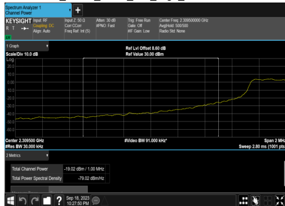
N30(5M)_DFT-s- OFDM_BPSK_Outer_Full_High_CH_CHP_PASS
