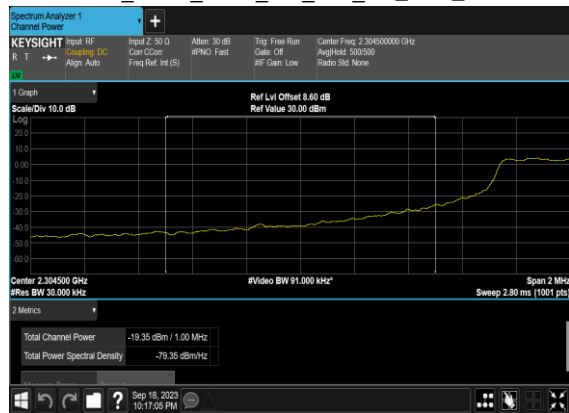
N30(5M)_DFT-s-OFDM_BPSK_Outer_Full_Low_CH_CHP_PASS
