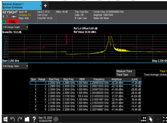
N30(10M)_DFT-s- OFDM_BPSK_Edge_1RB_Right_Low_CH
