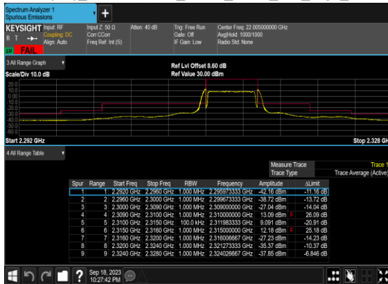
N30(5M)_DFT-s-OFDM_BPSK_Outer_Full_High_CH
