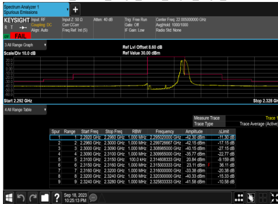
N30(5M)_DFT-s- OFDM_QPSK_Edge_1RB_Right_High_CH
