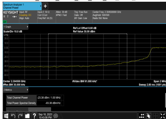
N30(10M)_DFT-s- OFDM_BPSK_Outer_Full_Low_CH_CHP_PASS
