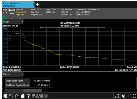
N30(5M)_DFT-s- OFDM_QPSK_Edge_1RB_Right_High_CH_CHP_PASS
