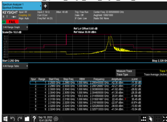
N30(10M)_DFT-s- OFDM_QPSK_Edge_1RB_Right_Low_CH
