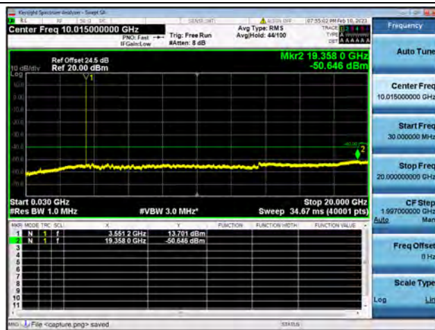
Band48-30M-20G / 15MHz / Low CH / 64QAM
