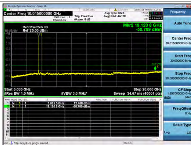
Band48-30M-20G / 20MHz / High CH / 64QAM
