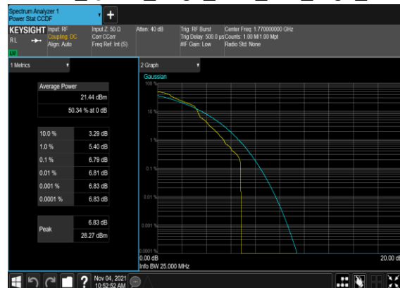
B5_N66(20M)_DFT-s- OFDM_QPSK_Edge_1RB_Left_High_CH
