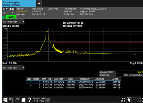
B12_N25(40M)_DFT-s- OFDM_QPSK_Edge_1RB_Right_High_CH
