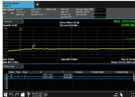
B12_N25(40M)_DFT-s-OFDM_QPSK_Edge_1RB_Left_Low_CH
