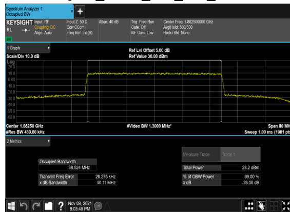
B12_N25(40M)_CP-OFDM_16 QAM_Outer_Full_Mid_CH
