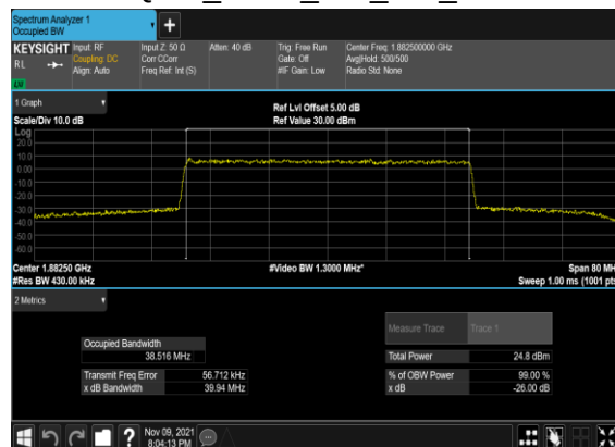
B12_N25(40M)_CP-OFDM_256 QAM_Outer_Full_Mid_CH
