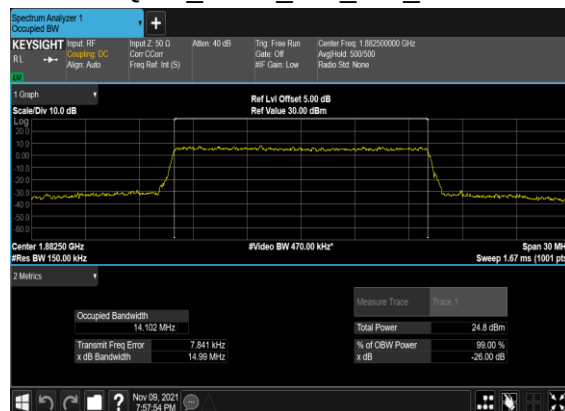
B12_N25(15M)_CP-OFDM_256 QAM_Outer_Full_Mid_CH
