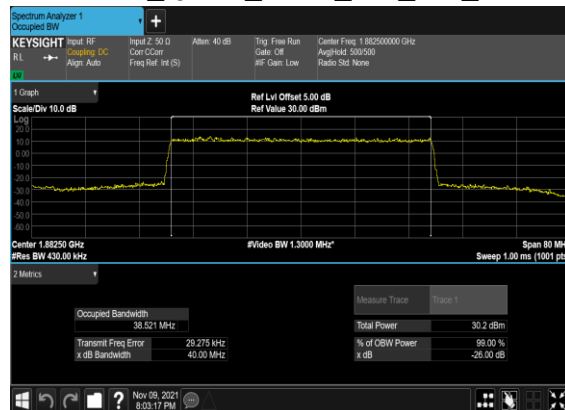
B12_N25(40M)_DFT-s- OFDM_QPSK_Outer_Full_Mid_CH
