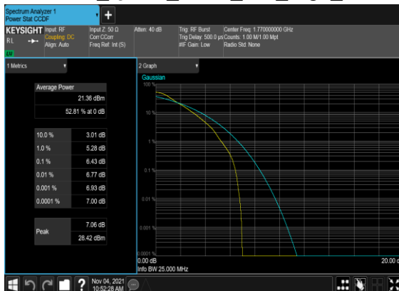
B5_N66(20M)_DFT-s- OFDM_QPSK_Outer_Full_High_CH
