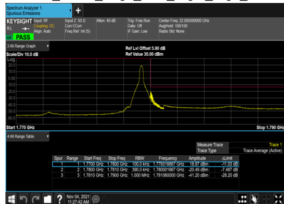
B5_N66(40M)_DFT-s- OFDM_BPSK_Edge_1RB_Right_High_CH
