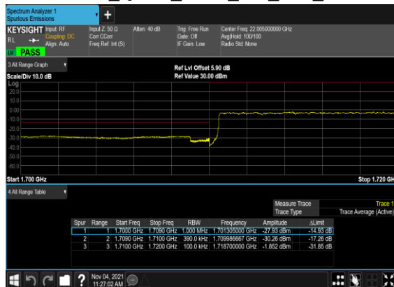
B5_N66(40M)_DFT-s- OFDM_QPSK_Outer_Full_Low_CH
