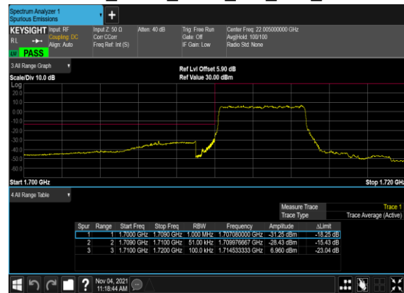
B5_N66(5M)_DFT-s-OFDM_BPSK_Outer_Full_Low_CH
