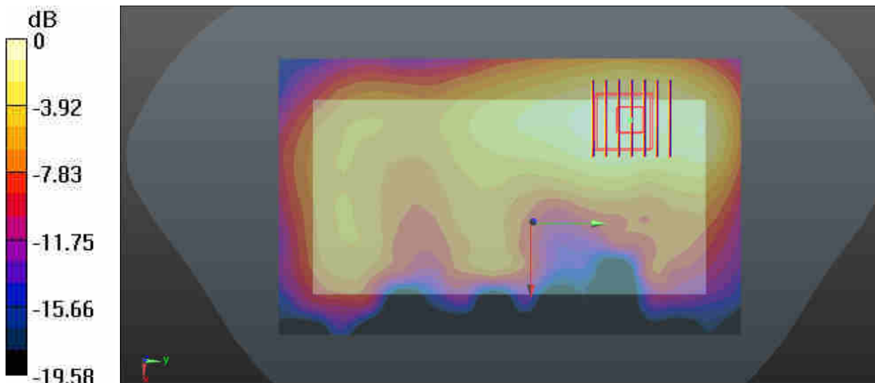
0 dB = 0.228 W/kg
