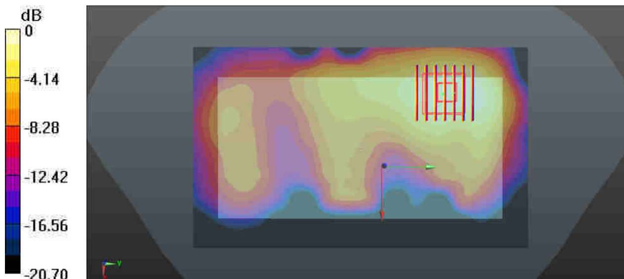
0 dB = 0.165 W/kg
