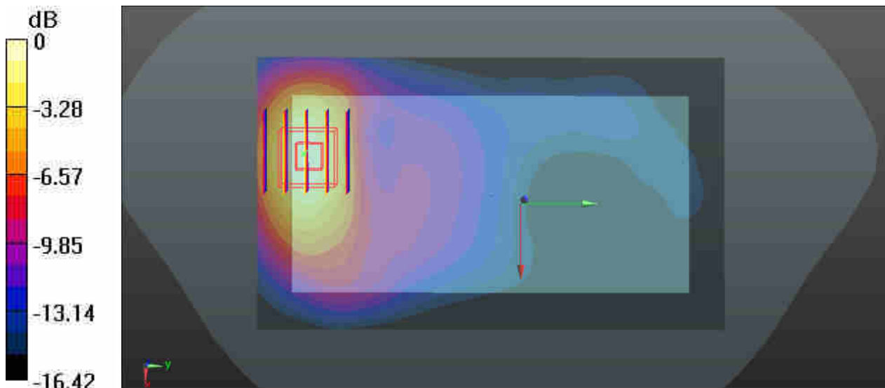
0 dB = 0.868 W/kg
