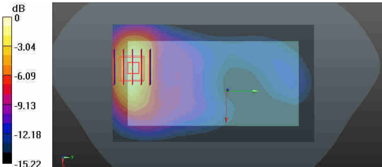
0 dB = 0.793 W/kg
