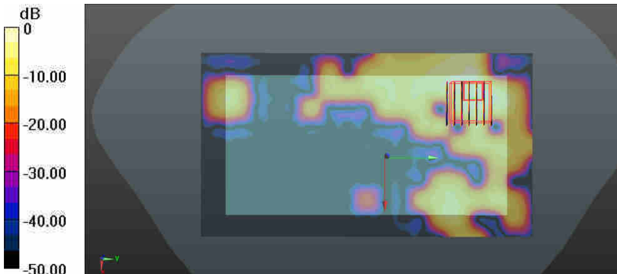
0 dB = 0.247 W/kg
