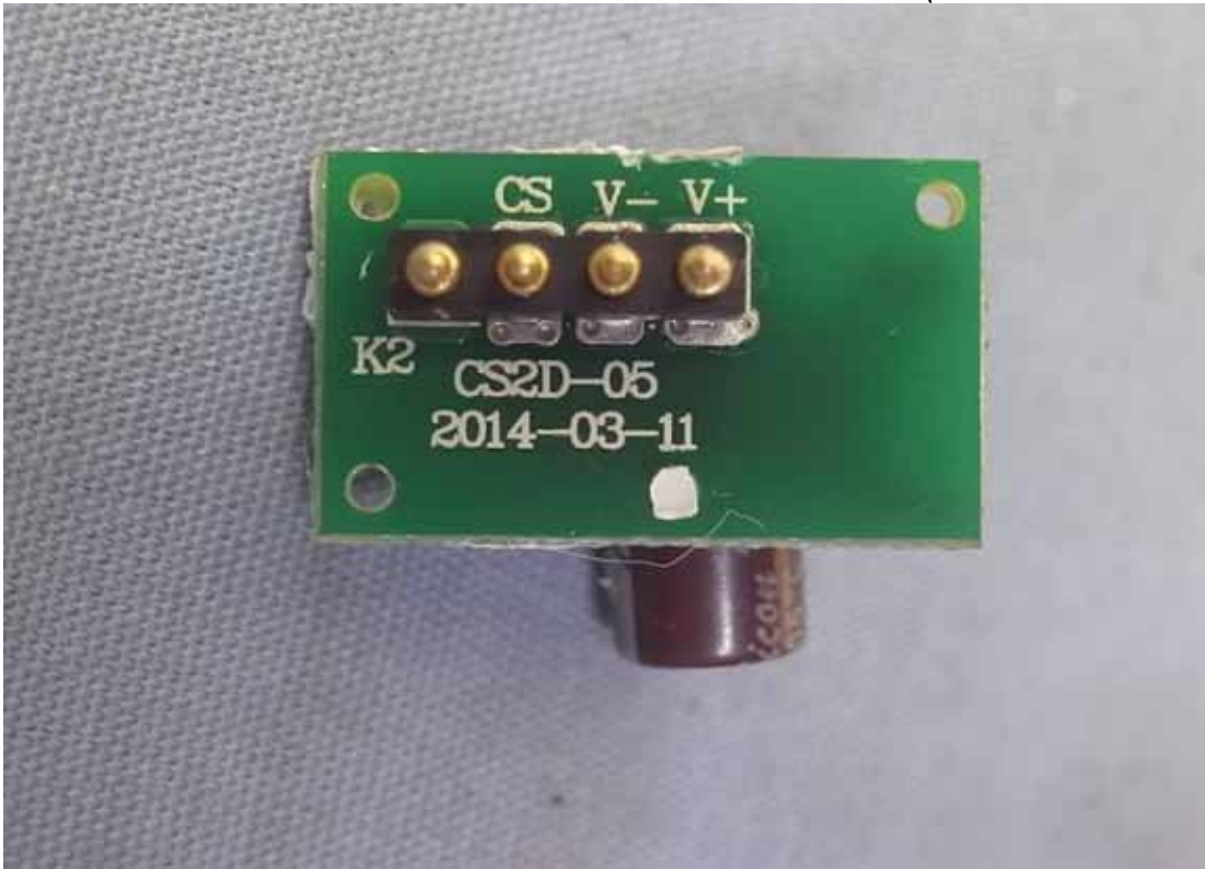
Figure 8 Internal View (Control Board/Front View)
