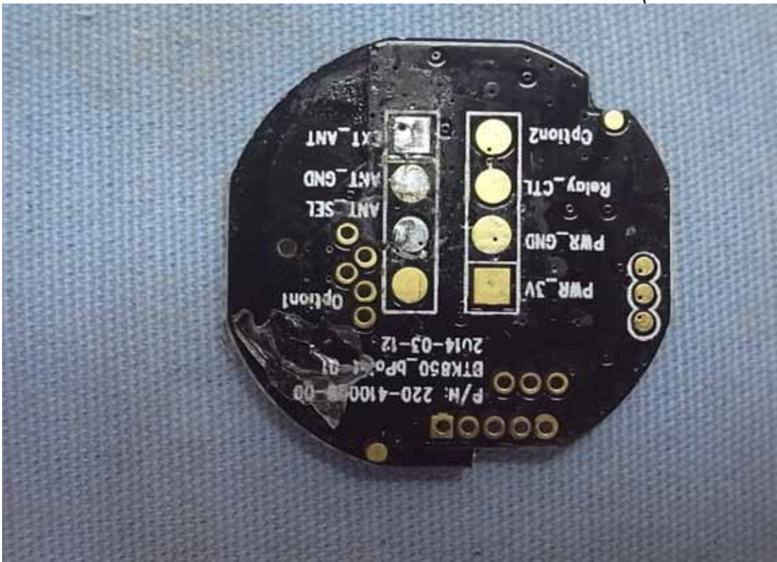
Figure 13 Internal View (RF Board/Back View)
