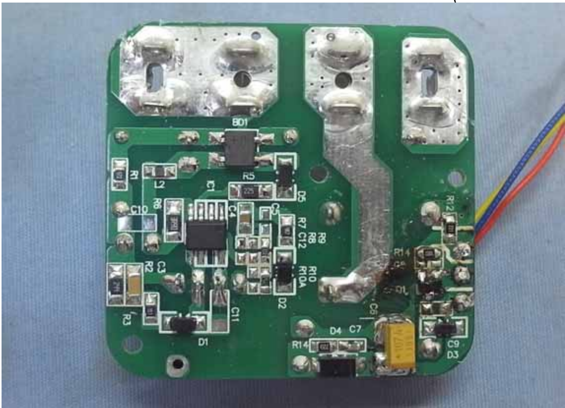
Figure 7 Internal View (Main Board/Back View)
