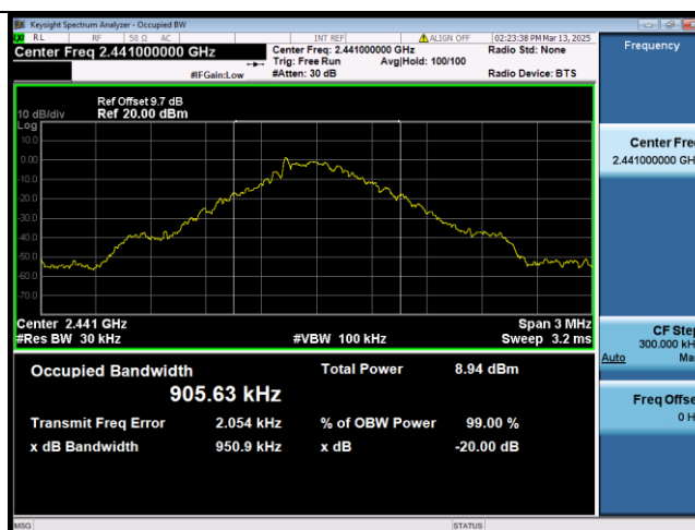
Bluetooth For Classic 2.4G 2441MHz
