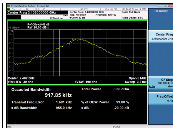
Bluetooth For Classic 2.4G 2402MHz
