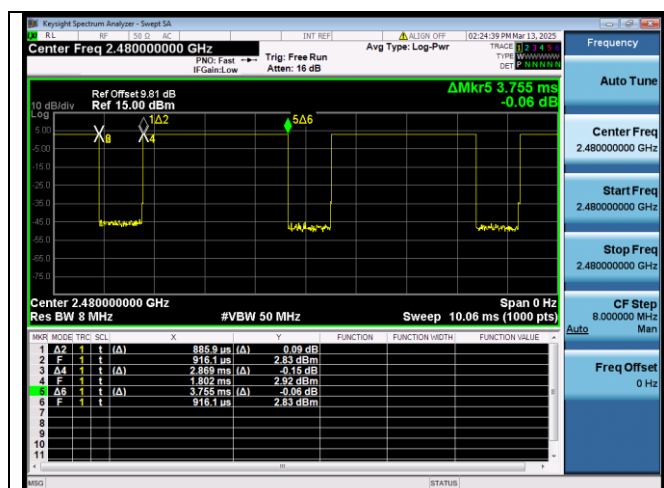
Bluetooth For Classic 2.4G 2480MHz
