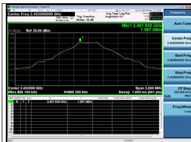
Bluetooth For Classic 2.4G
