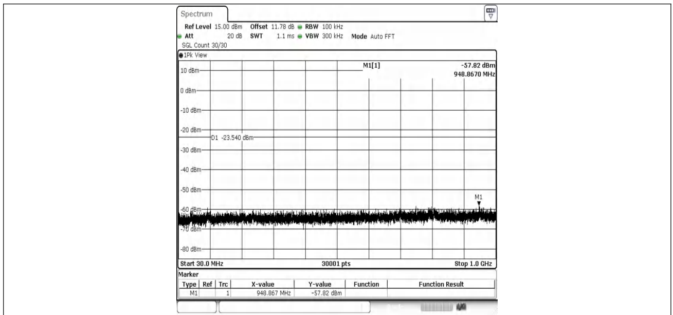
BLE_1M-Ant1-2440-30~1000-PASS
