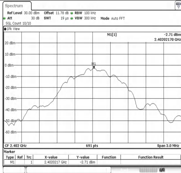
BLE_1M-Ant1-2402-0~Reference-PASS
