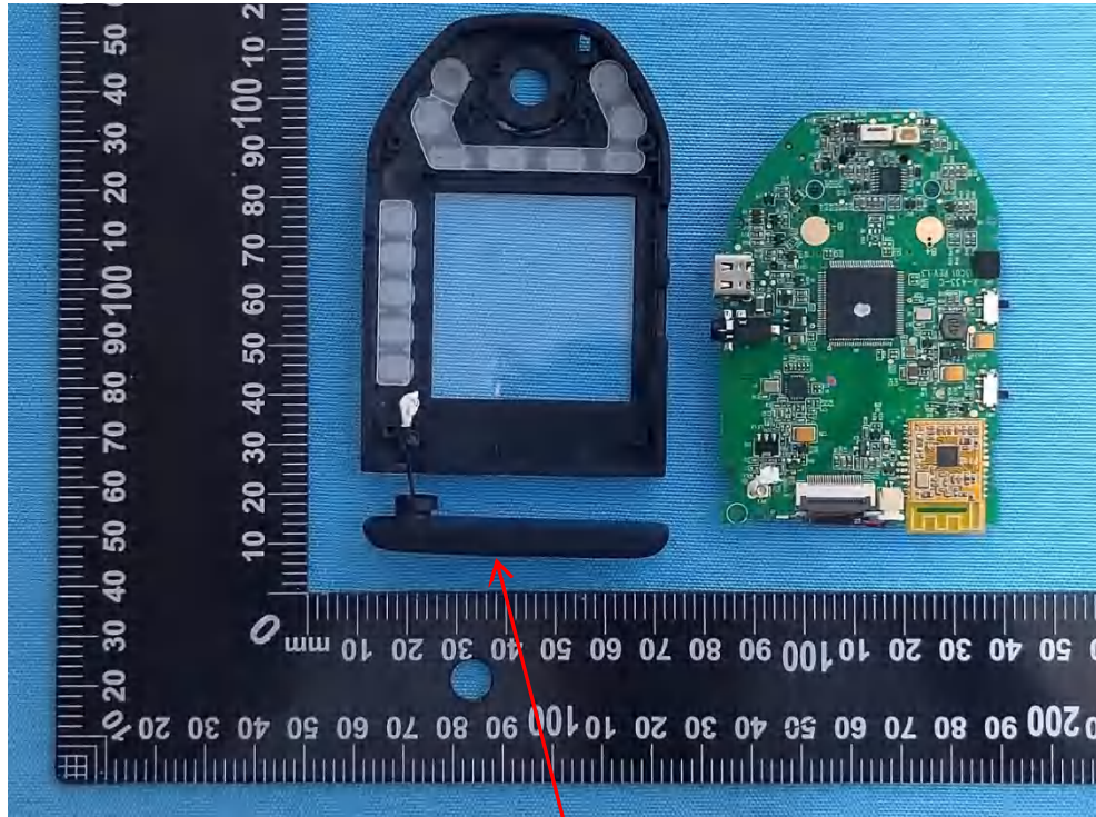
433 MHz-TX-ANT Location
