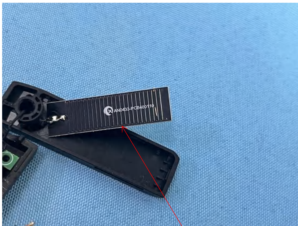
433MHz ANT
