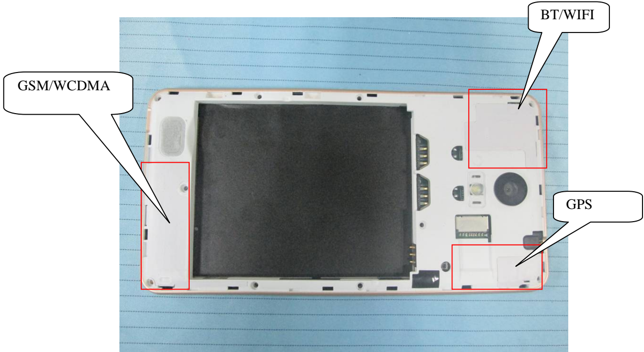
EUT –Antenna View
