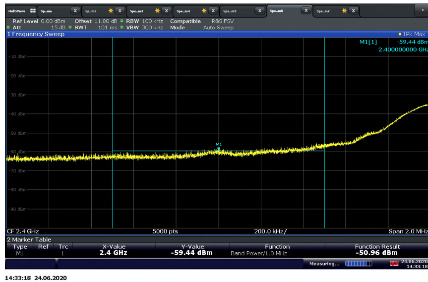
BT LE 1M Low Band Edge 2400MHz (Peak Measurement) @ Ch 2402 MHz (For reference only, not in the restricted band)
