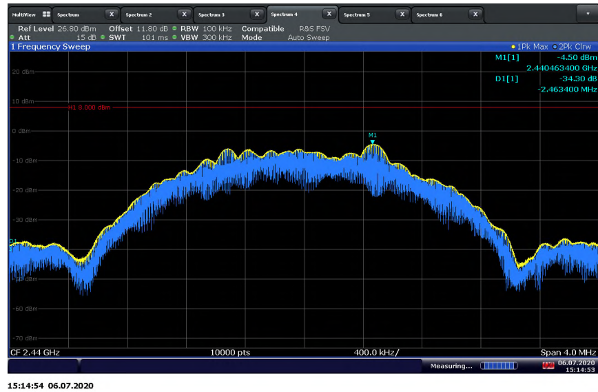
Bluetooth LE 2M Middle Channel
