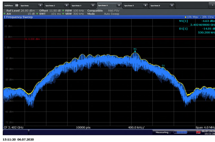
Bluetooth LE 2M Low Channel
