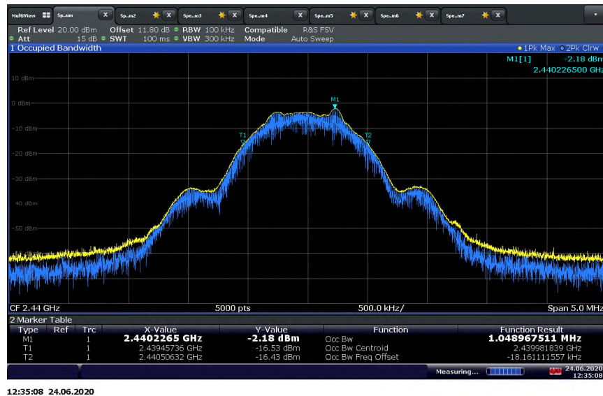
Bluetooth LE 1M Middle Channel
