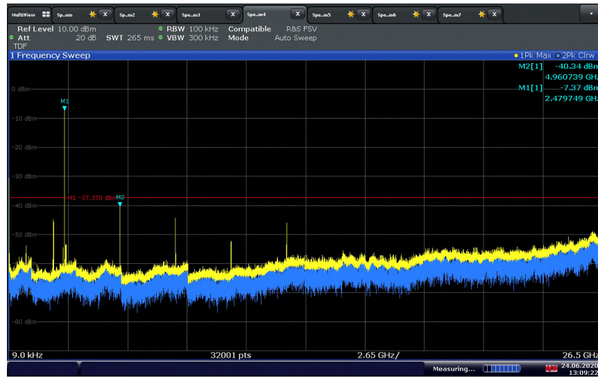
Bluetooth LE 2M High Channel
