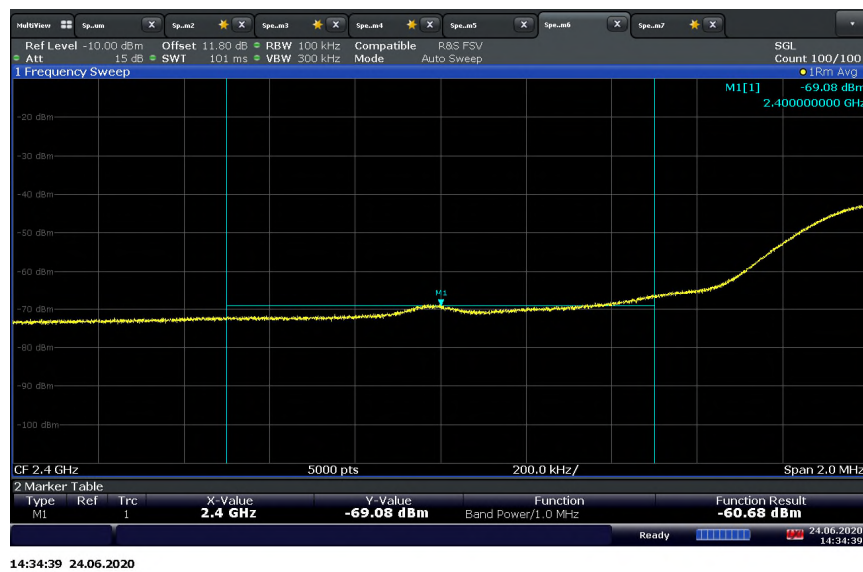
BT LE 1M Low Band Edge (Average Measurement). Limit is -33.03 dBm. Margin is -27.65 dB. (The highest level of the desired power within the band is -3.03 dBm)
