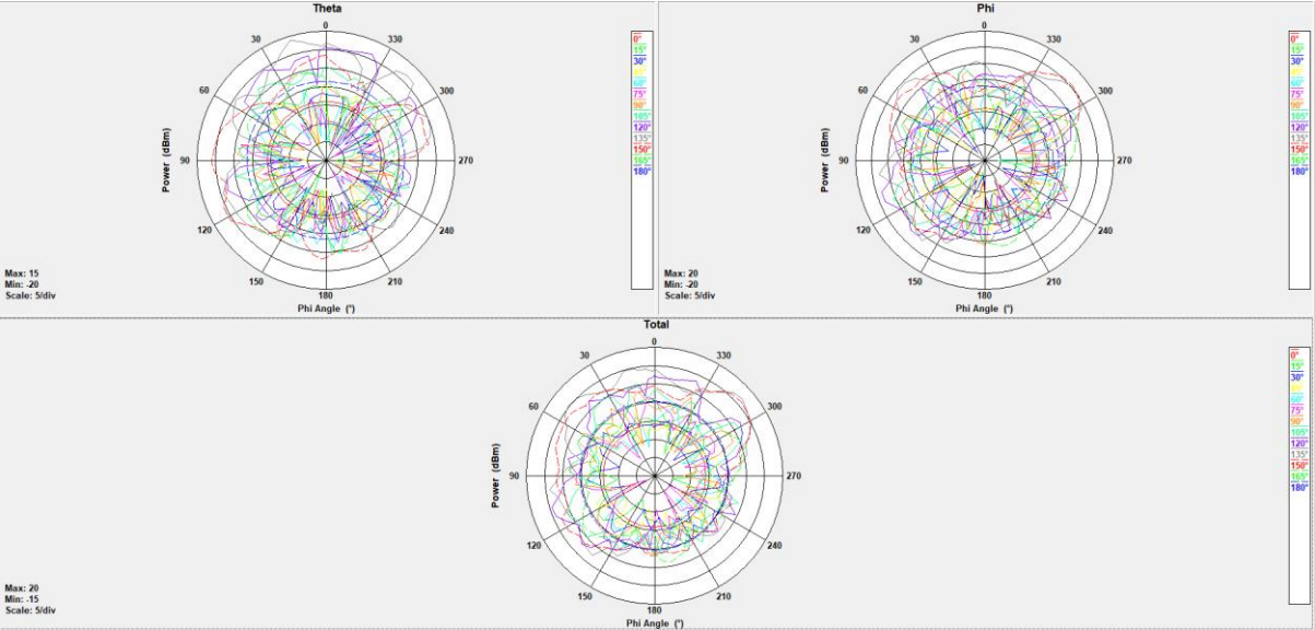
Figure 5. CHAIN2, 5GHz
