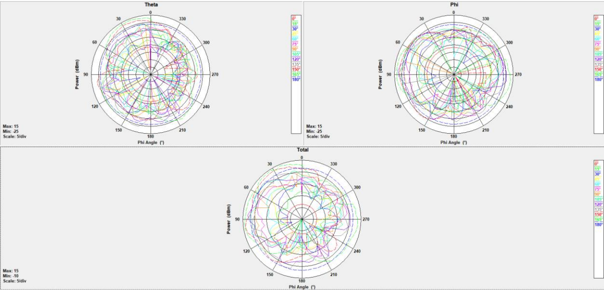
Figure 2. CHAIN1, 2.4GHz
