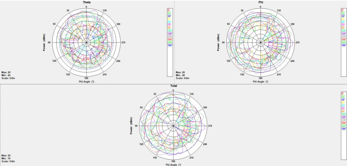
Figure 4. CHAIN1, 5GHz
