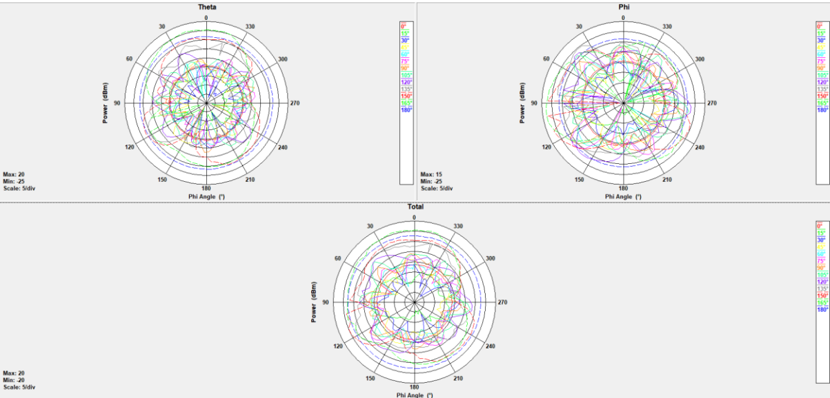
Figure 3. CHAIN2, 2.4GHz
