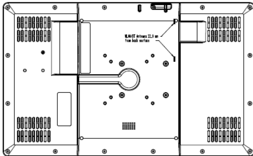
Figure 1. WLAN Antenna locations (Back)
