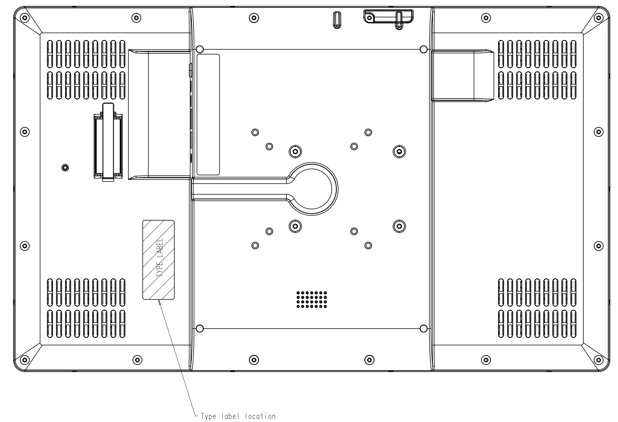
BACK VIEW
