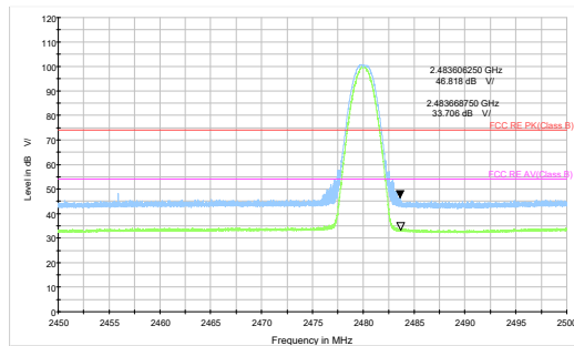
Bluetooth LE (S=8) Channel 39 Peak+ Average
