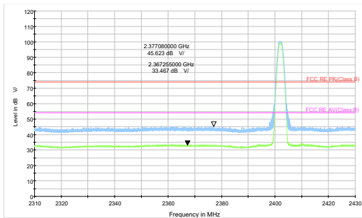
Bluetooth LE (S=8) Channel 0 Peak+ Average
