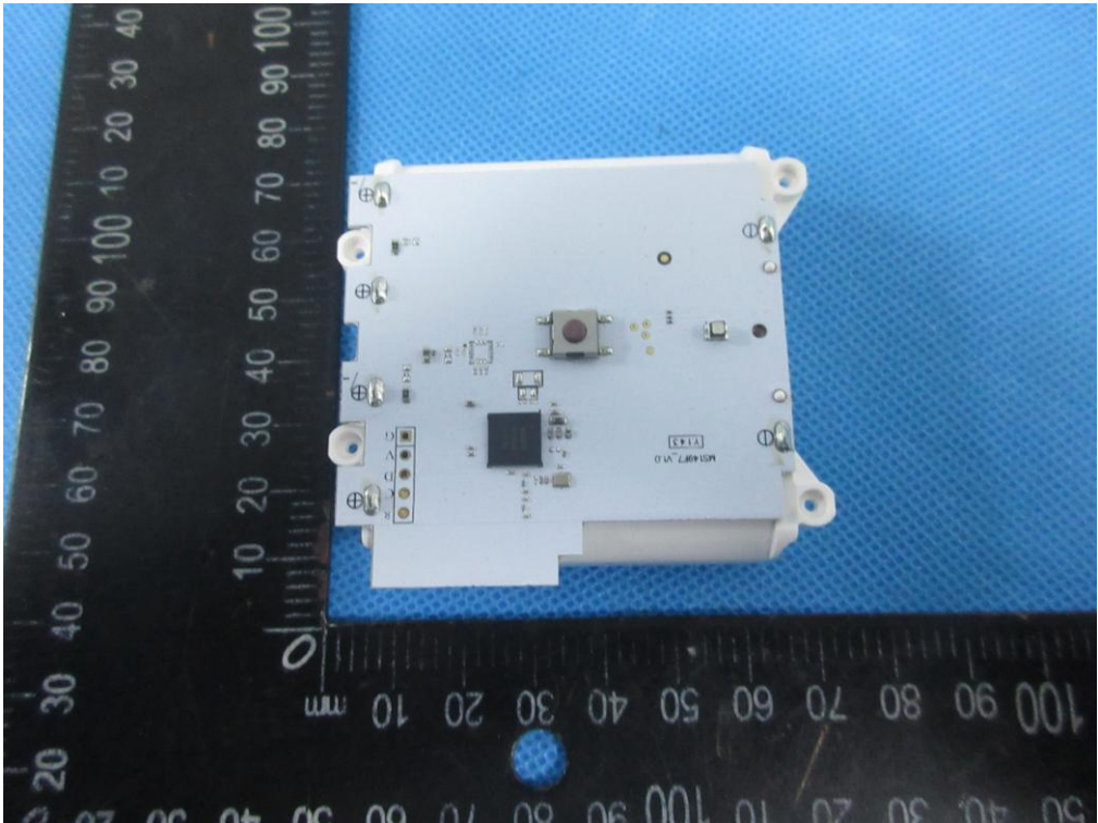
Photo 10 (parallel connection)
