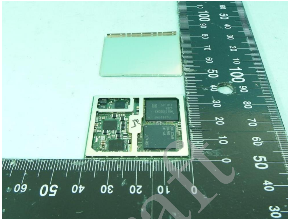
(1) EUT Photo
