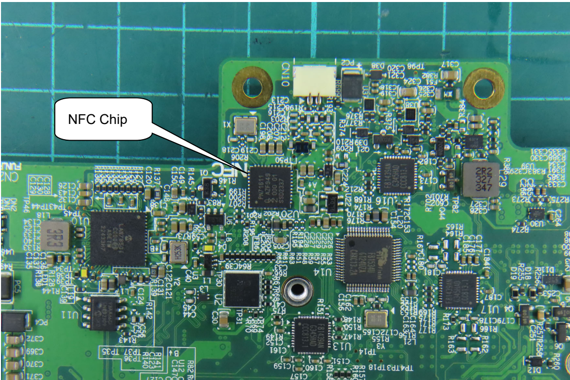
(25) EUT Photo
