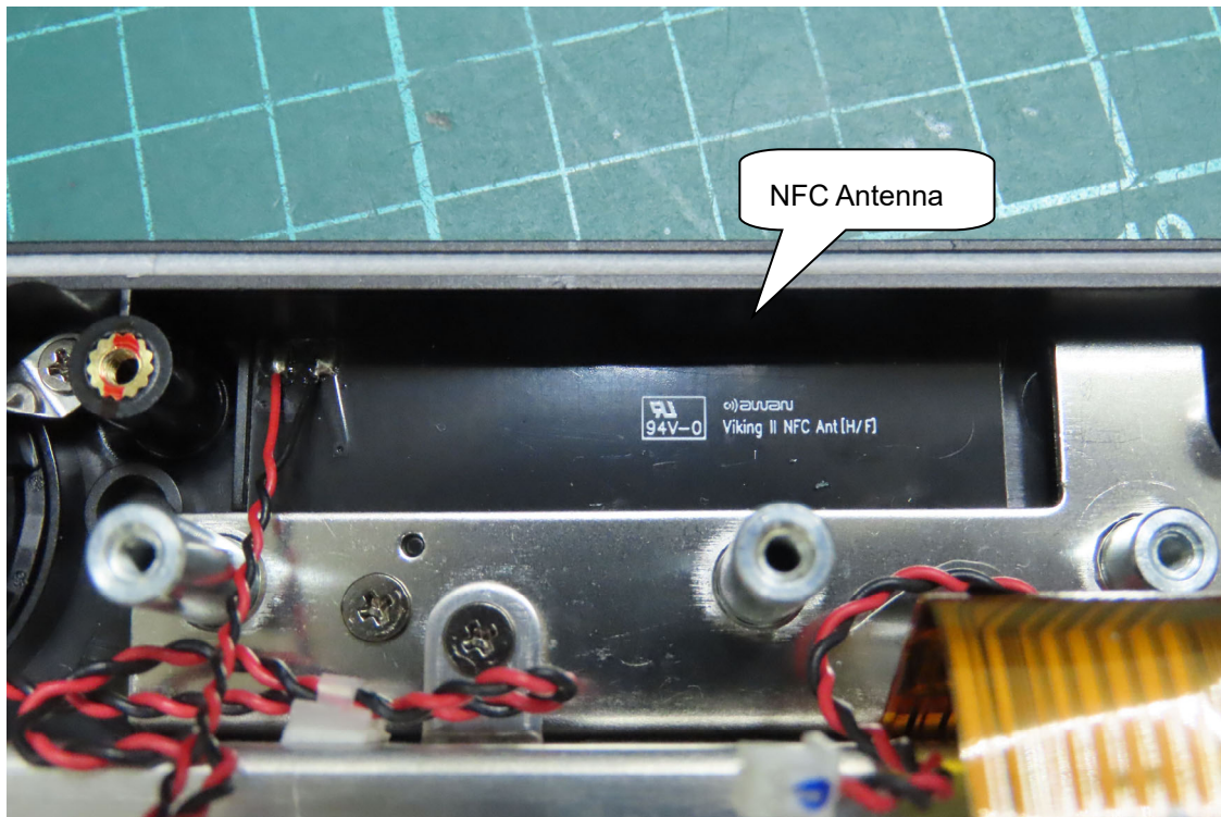
(29) EUT Photo
