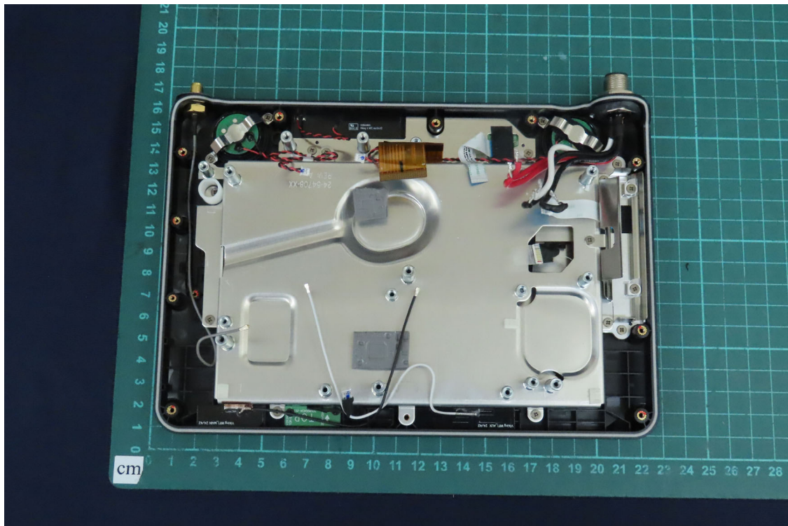
(26) EUT Photo
