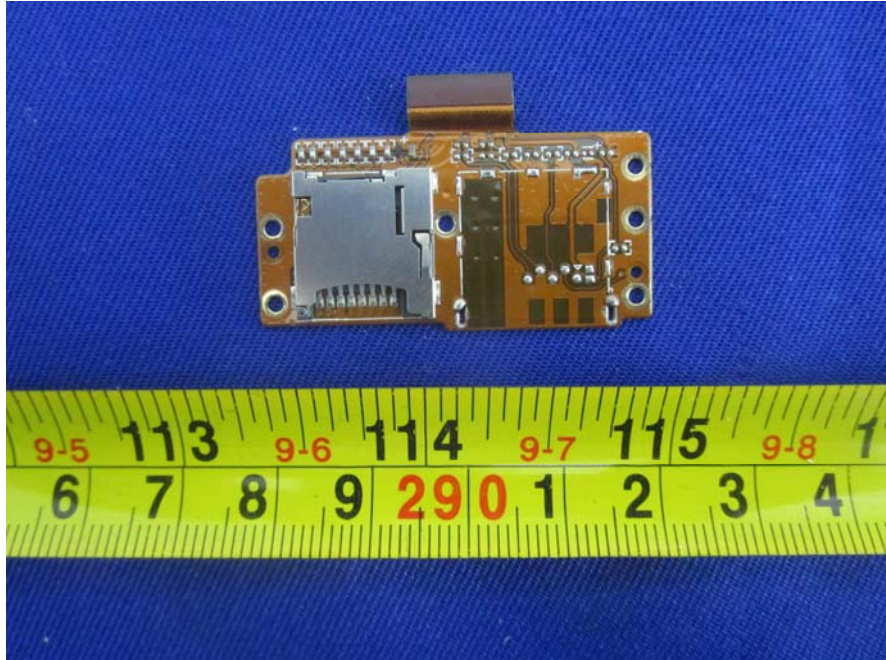
EUT – TF Card Board Top View
