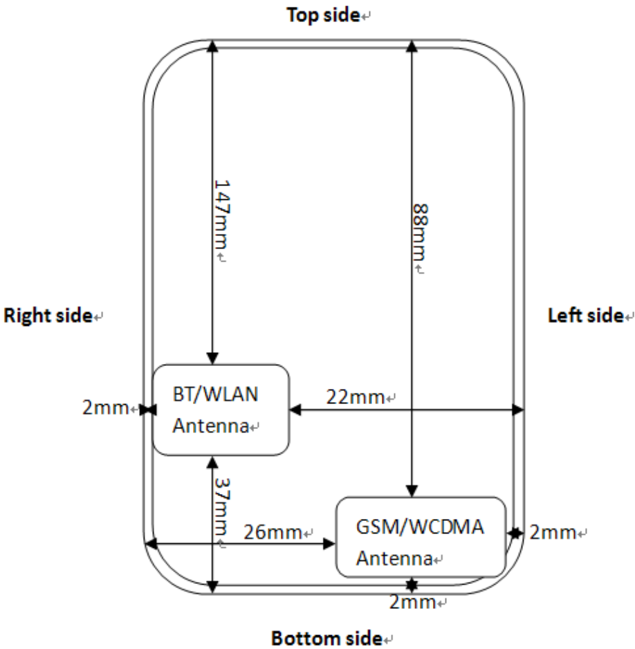
Figure 2:The antenna positions of the DUT
