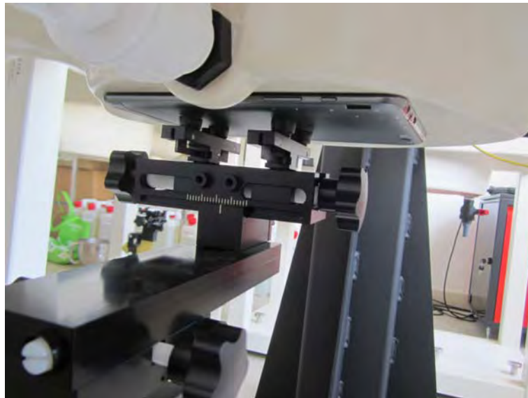
Body- worn Front side Photo(0mm to Phantom)
