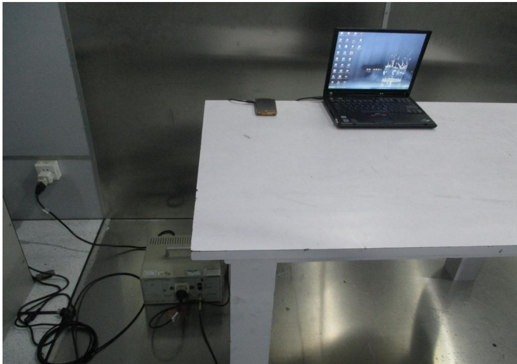
Conducted Test setup photo
