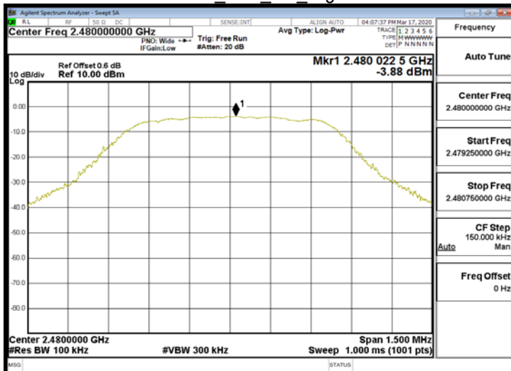
Reference Level BLE 1M HighCH39-2480
