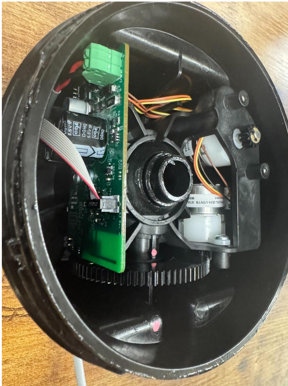
Bottom Part (Electronics Housing)
