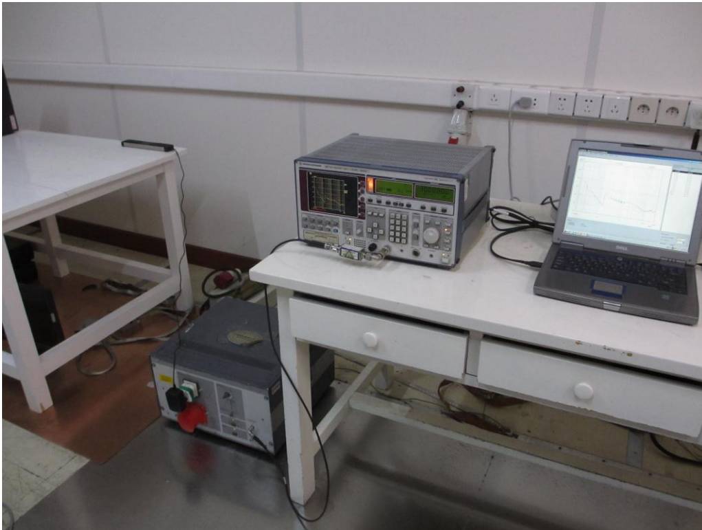
Photograph 4: Set-up for RF test
