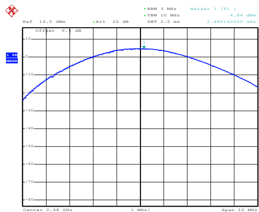
Highest channel
