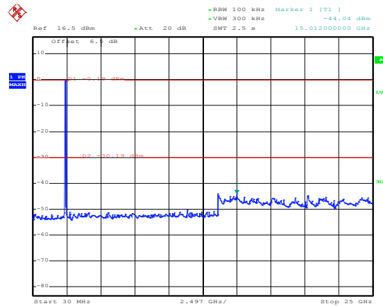
Test mode: 802.11n(HT40) Lowest channel
