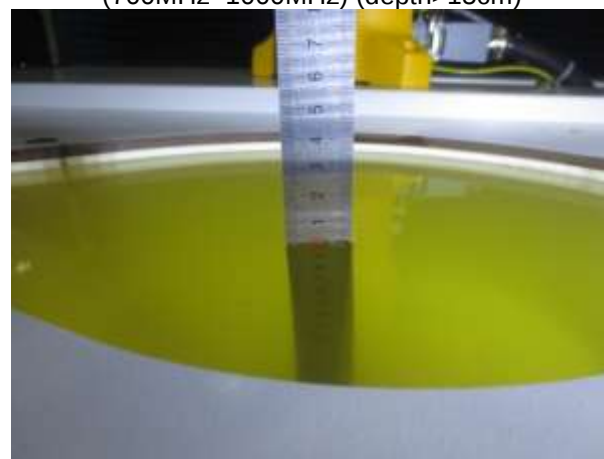
Fig. 9.4 Photo of Liquid Height for Body SAR (1710MHz~1910MHz) (depth>15cm)
