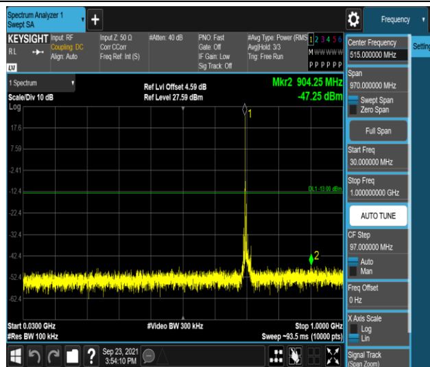
Band12-10MHz-16QAM-23095-1RB#0-Range1:30~1000MHz
