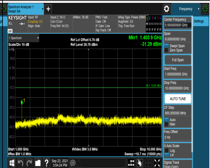
Band12-10MHz-16QAM-23095-1RB#0-Range2:1000~10000MHz
