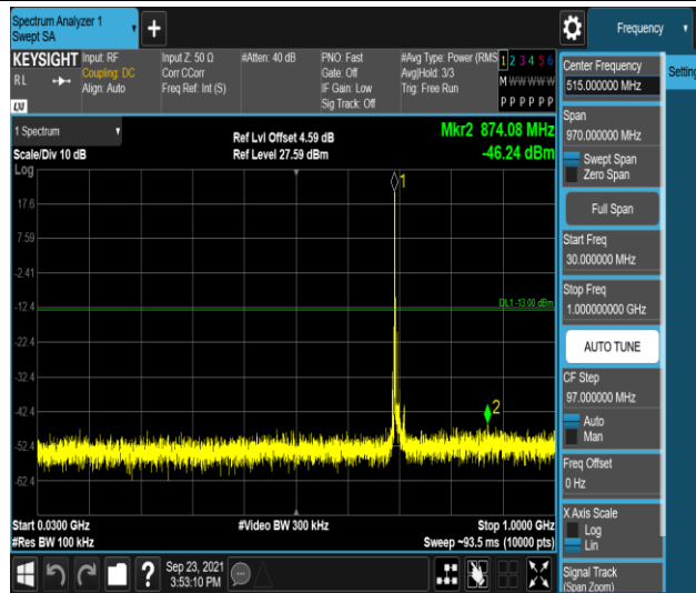
Band12-10MHz-16QAM-23060-1RB#0-Range1:30~1000MHz
