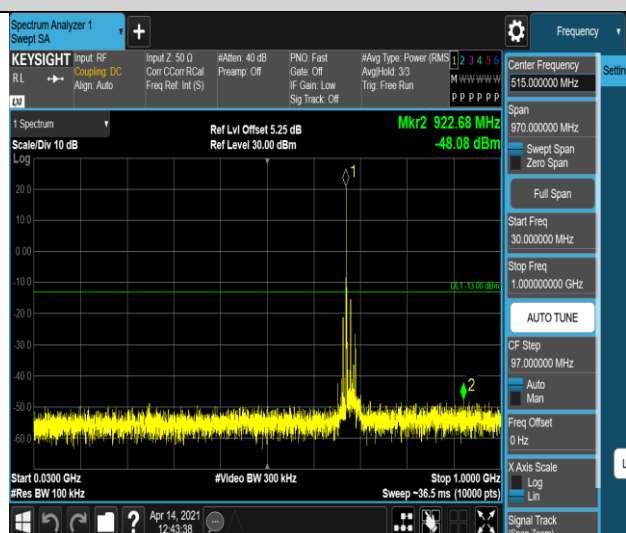
Band71-20MHz-16QAM-133222-1RB#0-Range1:30~ ~1000MHz
