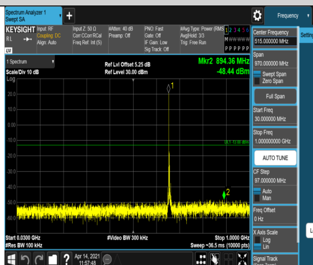
Band71-5MHz-16QAM-133297-1RB#0-Range1:30~ 1000MHz
