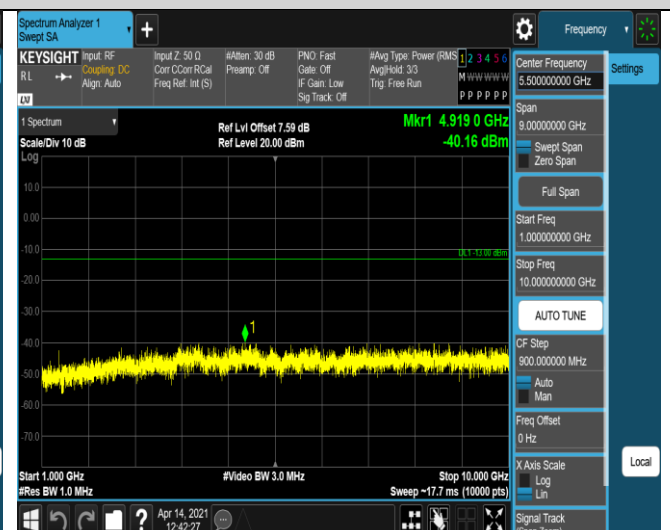
Band71-20MHz-16QAM-133322-1RB#0-Range2:1000~ 10000MHz
