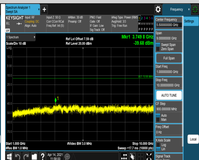
Band71-5MHz-16QAM-133297-1RB#0-Range2:1000~1 0000MHz
