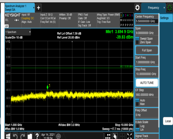
Band71-5MHz-16QAM-133447-1RB#0-Range2:1000~1 0000MHz
