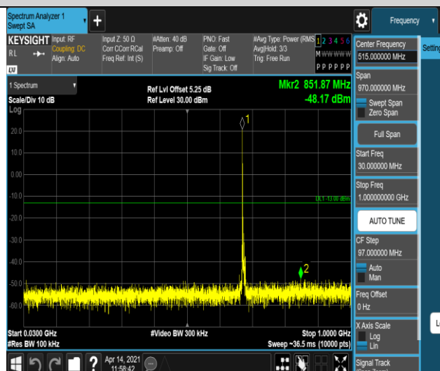
Band71-5MHz-16QAM-133447-1RB#0-Range1:30~ 1000MHz
