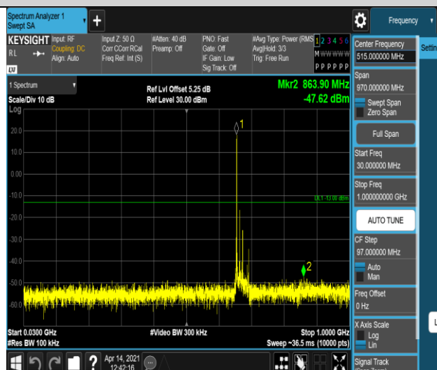
Band71-20MHz-16QAM-133322-1RB#0-Range1:30~ ~1000MHz
