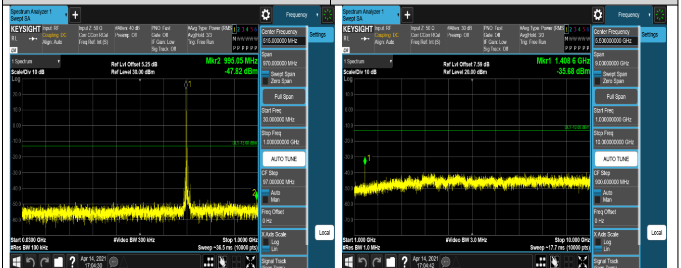
Band17-10MHz-QPSK-23780-1RB#0-Range1:30~1
