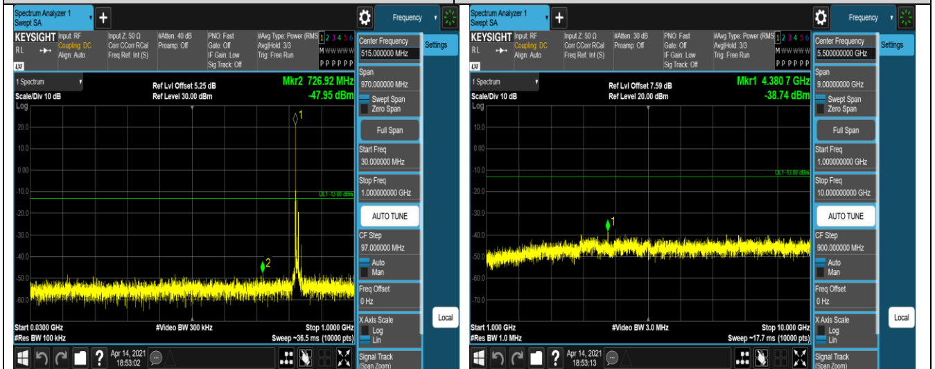
Band5-10MHz-16QAM-20525-1RB#0-Range1:30~1
