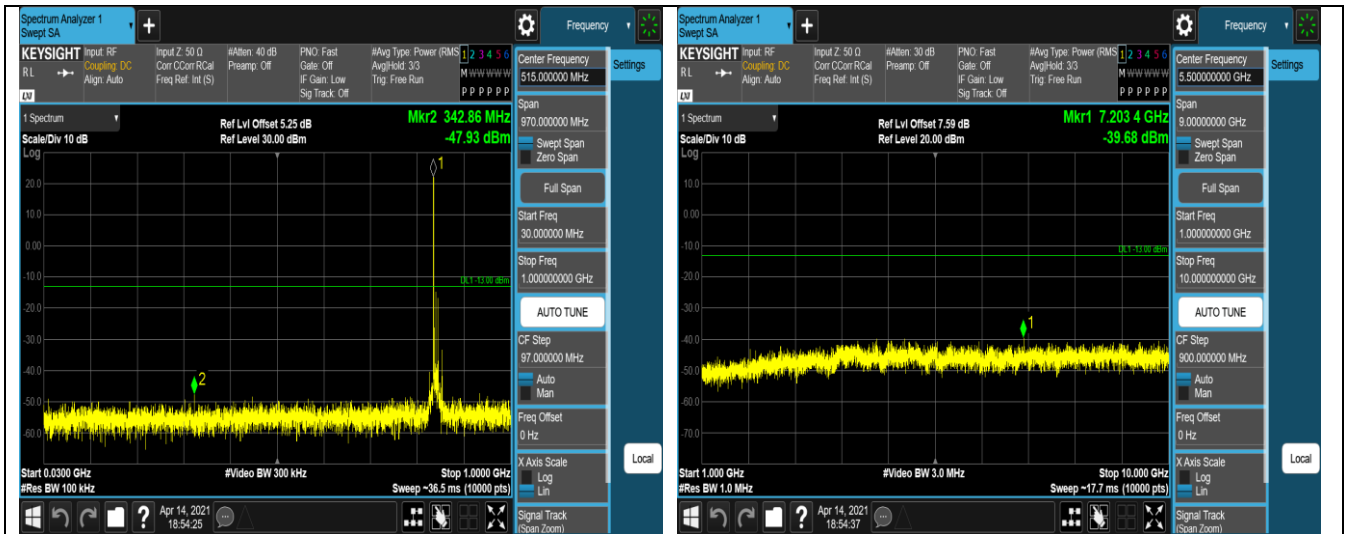
Band5-10MHz-16QAM-20450-1RB#0-Range1:30~1
