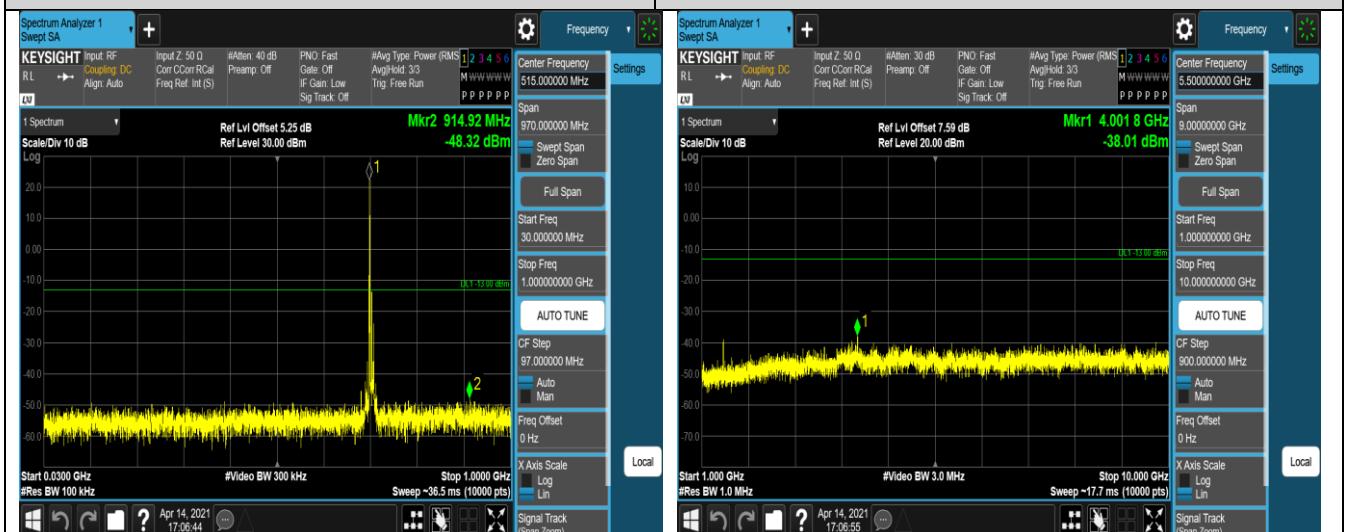
Band17-10MHz-16QAM-23800-1RB#0-Range1:30~1000MHz
