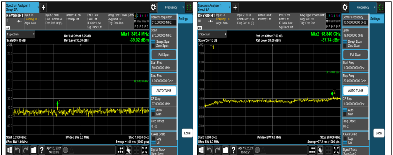
Band2-1.4MHz-16QAM-18607-1RB#0-Range1:30~1000MHz
