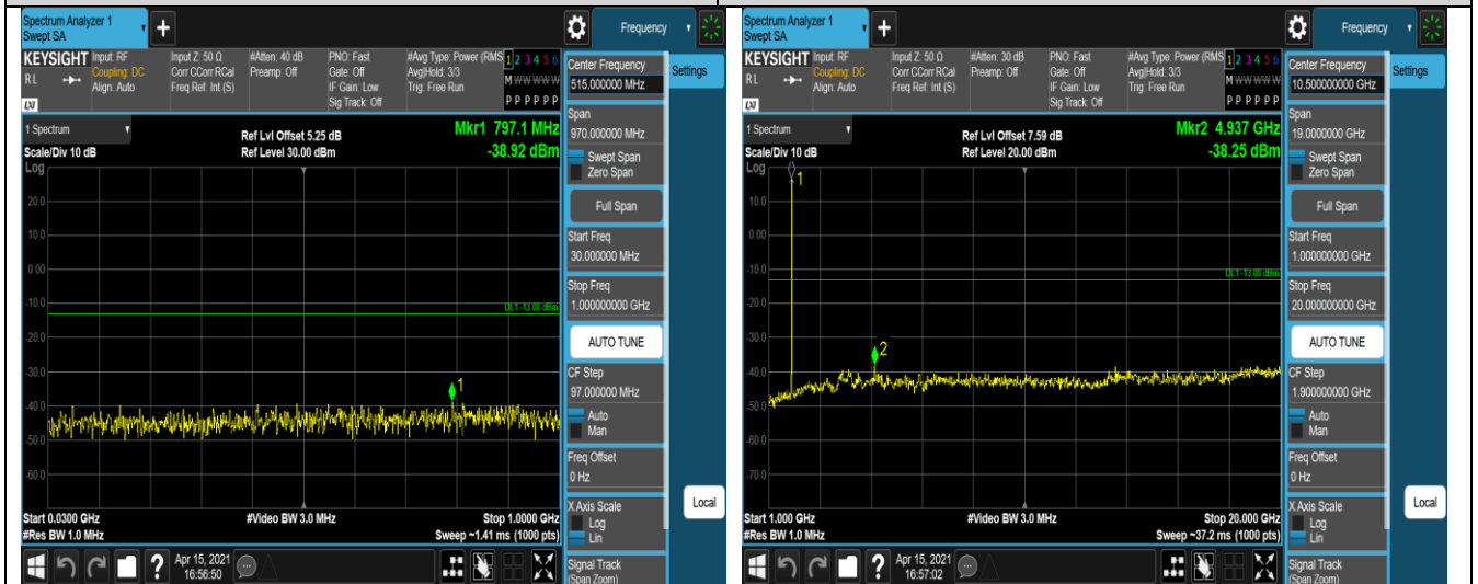
Band2-1.4MHz-16QAM-18900-1RB#0-Range1:30~1000MHz
