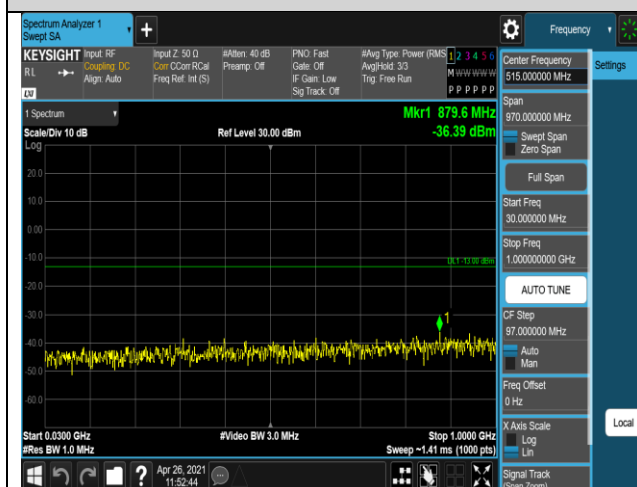
Band5-1.4MHz-QPSK-20407-1RB#0-Range1:30~10
