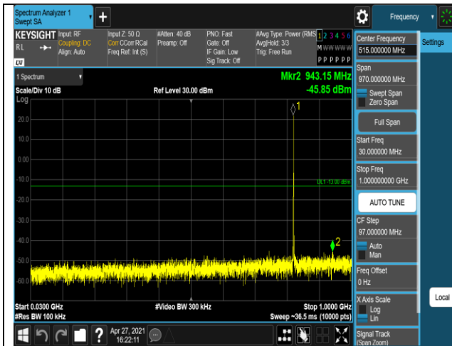
Band5-1.4MHz-QPSK-20525-1RB#0-Range1:30~10
