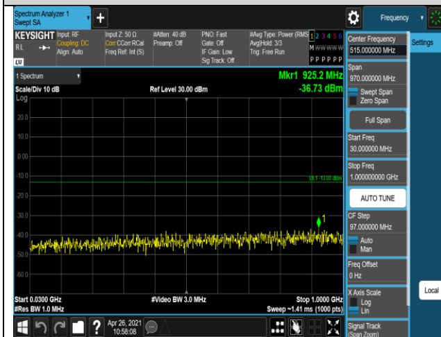
Band4-1.4MHz-16QAM-20393-1RB#0-Range1:30~1000MHz
