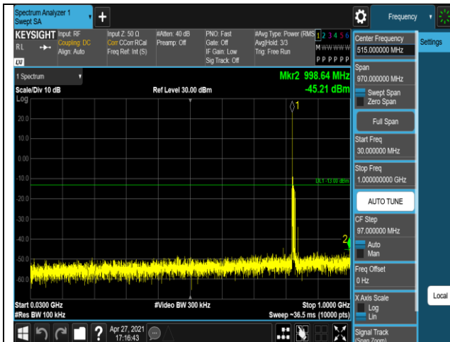
Band5-10MHz-QPSK-20525-1RB#0-Range1:30~10
