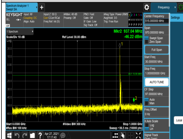
Band5-10MHz-QPSK-20600-1RB#0-Range1:30~10
