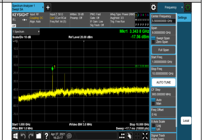
Band5-1.4MHz-QPSK-20643-1RB#0-Range2:1000~10
