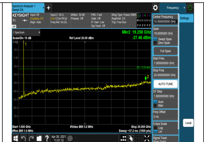
Band4-20MHz-16QAM-20175-1RB#0-Range2:1000~20
