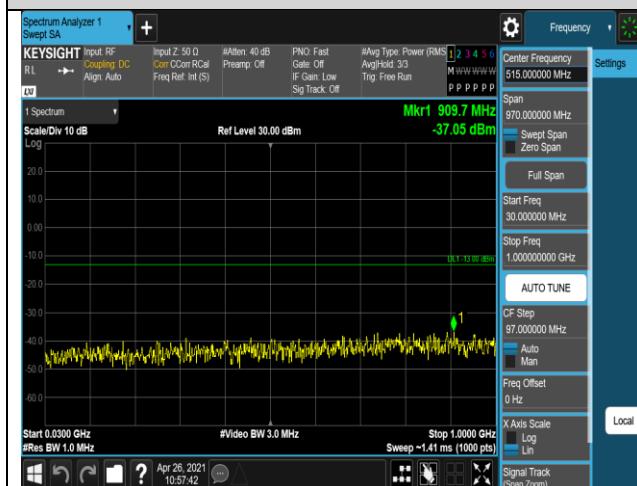
Band4-1.4MHz-QPSK-20393-1RB#0-Range1:30~10
