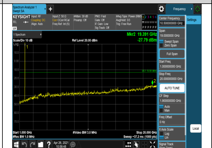
Band4-1.4MHz-16QAM-19957-1RB#0-Range2:1000~2
