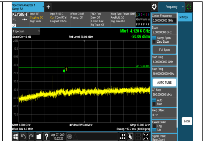
Band5-1.4MHz-QPSK-20525-1RB#0-Range2:1000~10
