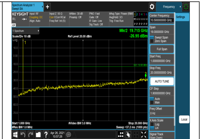
Band4-1.4MHz-16QAM-20175-1RB#0-Range2:1000~20000MHz
