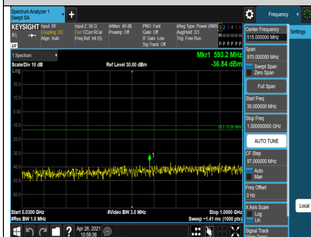
Band4-1.4MHz-16QAM-19957-1RB#0-Range1:30~1
