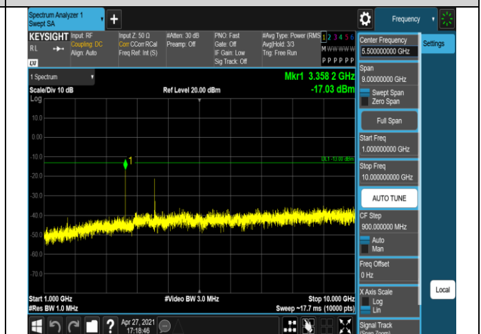
Band5-10MHz-16QAM-20450-1RB#0-Range2:1000~10
