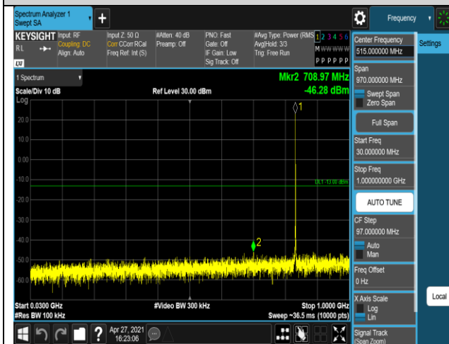
Band5-1.4MHz-QPSK-20643-1RB#0-Range1:30~10
