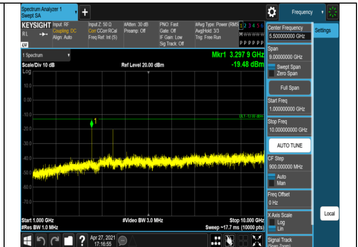
Band5-10MHz-QPSK-20525-1RB#0-Range2:1000~100
