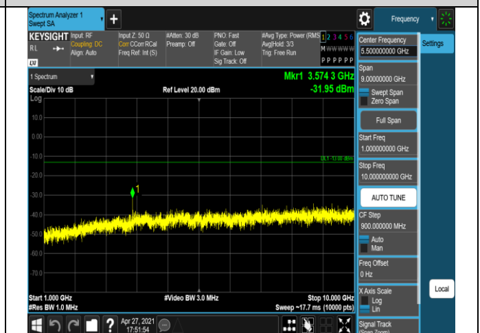
Band12-1.4MHz-16QAM-23017-1RB#0-Range2:1000~10000MHz
