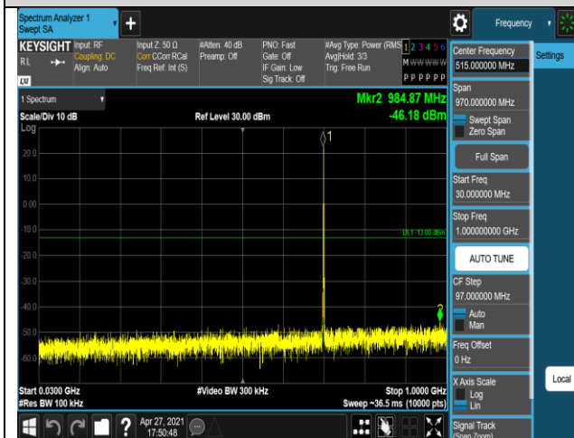
Band12-1.4MHz-QPSK-23173-1RB#0-Range1:30~1000MHz
