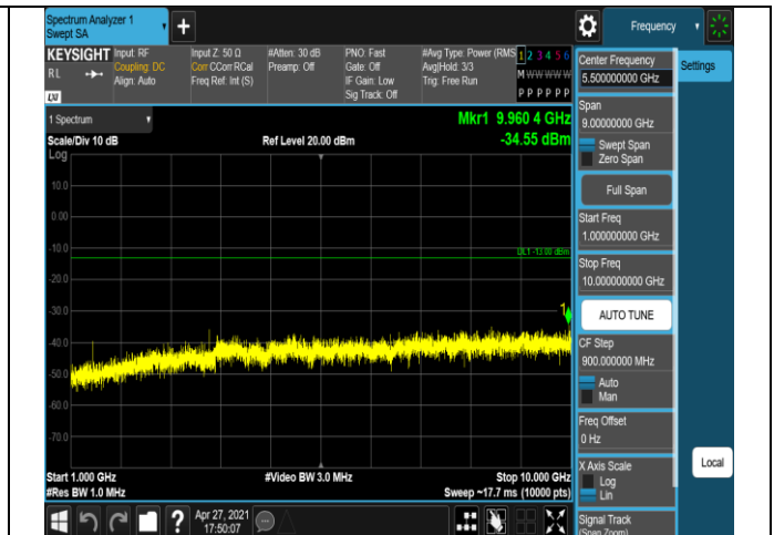
Band12-1.4MHz-QPSK-23095-1RB#0-Range2:1000~10000MHz
