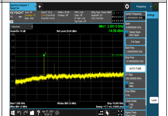
Band5-1.4MHz-16QAM-20407-1RB#0-Range2:1000~1
