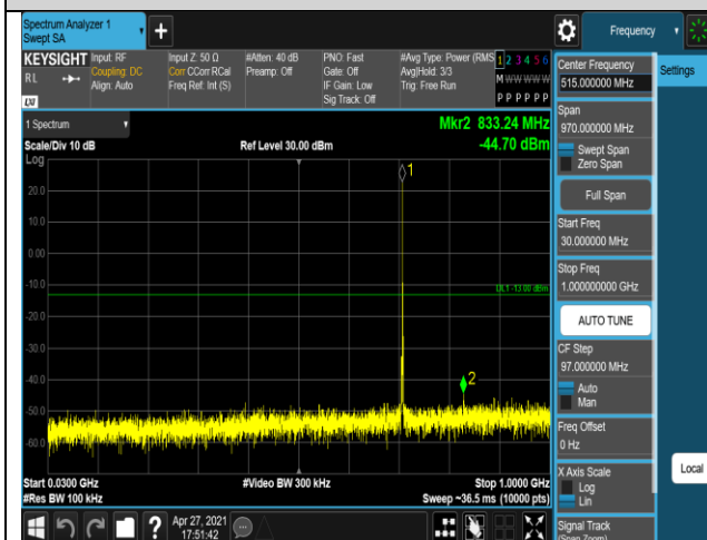
Band12-1.4MHz-16QAM-23017-1RB#0-Range1:30~1000MHz
