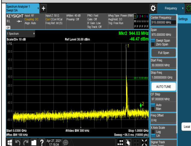
Band5-10MHz-16QAM-20450-1RB#0-Range1:30~1
