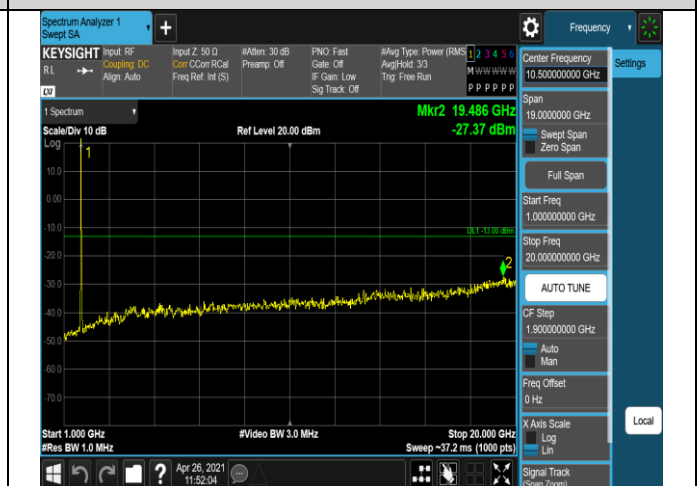
Band4-20MHz-16QAM-20300-1RB#0-Range2:1000~20
