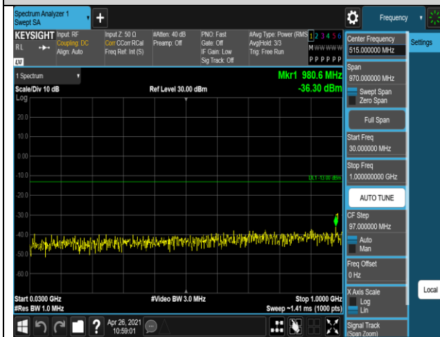
Band4-20MHz-QPSK-20050-1RB#0-Range1:30~1000MHz
