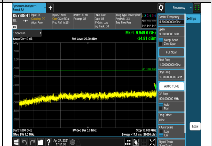
Band12-1.4MHz-QPSK-23173-1RB#0-Range2:1000~10000MHz
