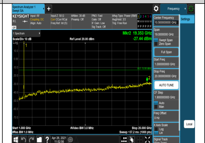
Band5-1.4MHz-QPSK-20407-1RB#0-Range2:1000~10
