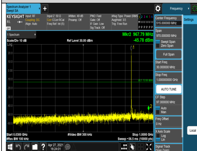
Band5-1.4MHz-16QAM-20407-1RB#0-Range1:30~1
