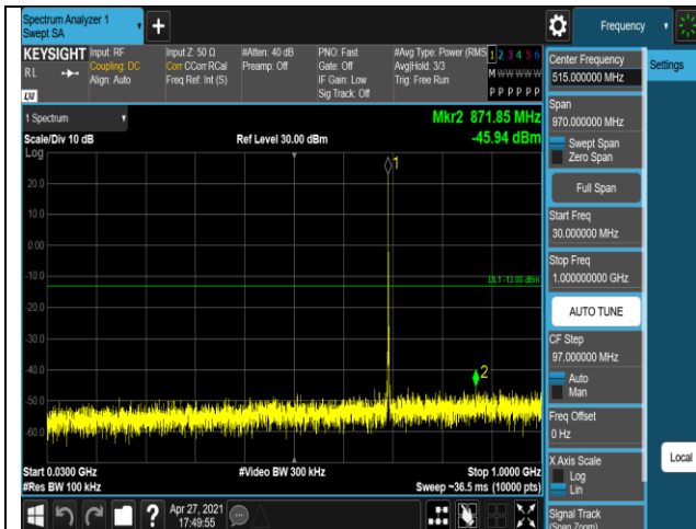
Band12-1.4MHz-QPSK-23095-1RB#0-Range1:30~1000MHz
