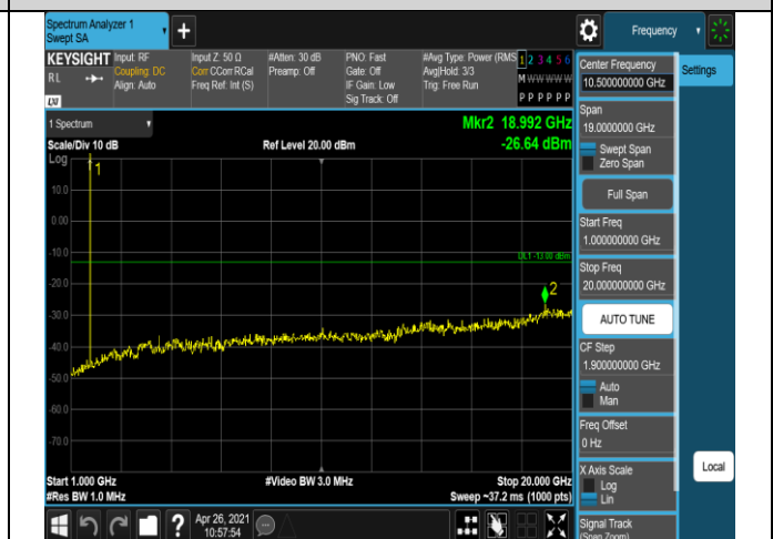
Band4-1.4MHz-QPSK-20393-1RB#0-Range2:1000~20
