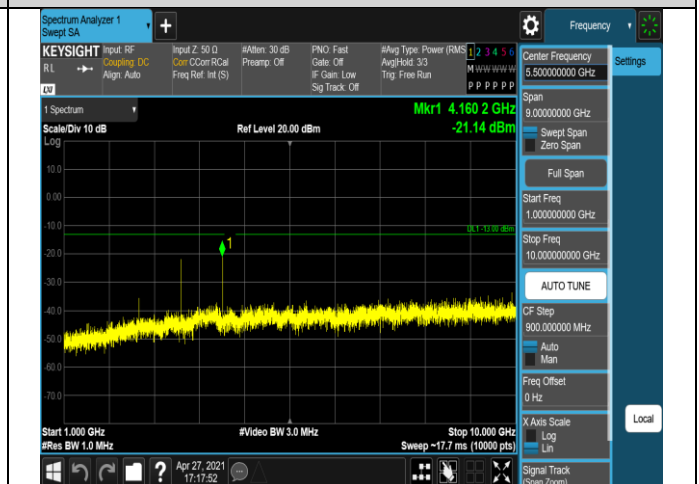
Band5-10MHz-QPSK-20600-1RB#0-Range2:1000~100
