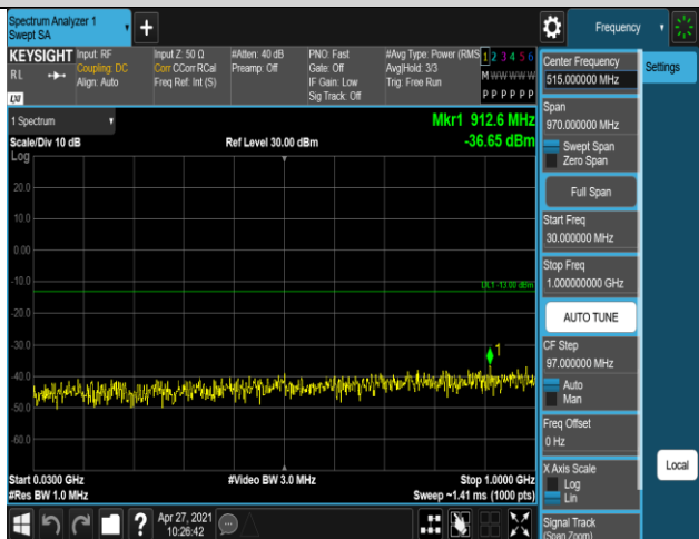
Band2-1.4MHz-16QAM-19193-1RB#0-Range1:30~1
