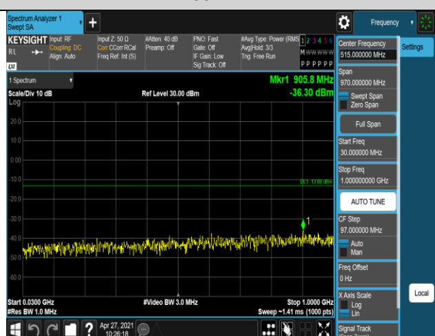
Band2-1.4MHz-QPSK-19193-1RB#0-Range1:30~1000MHz
