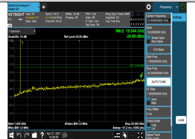
Band2-1.4MHz-16QAM-19193-1RB#0-Range2:1000~2
