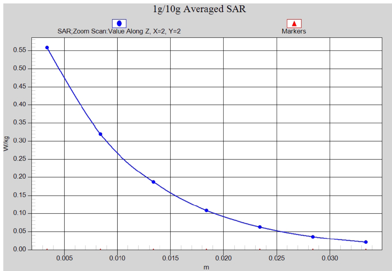
Z-Scan at power reference point- Body- worn Rear Side (WiFi2450 Middle Channel-Channel 6-2437MHz (1Mbps))
