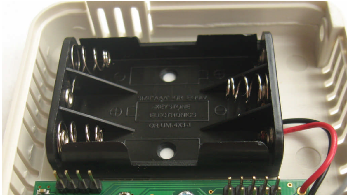
Fig. 4 Empty Battery Holder
