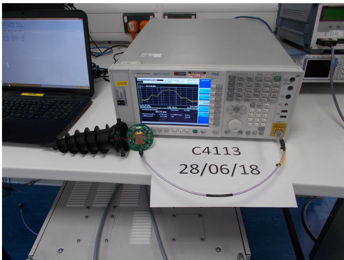
Antenna Port conducted Test (6dB Bandwidth)
