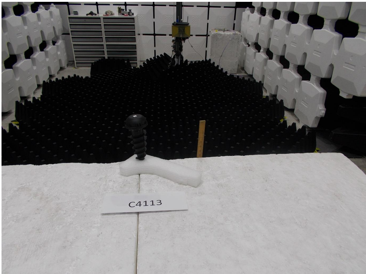
Radiated emissions 1GHz to 10GHz
