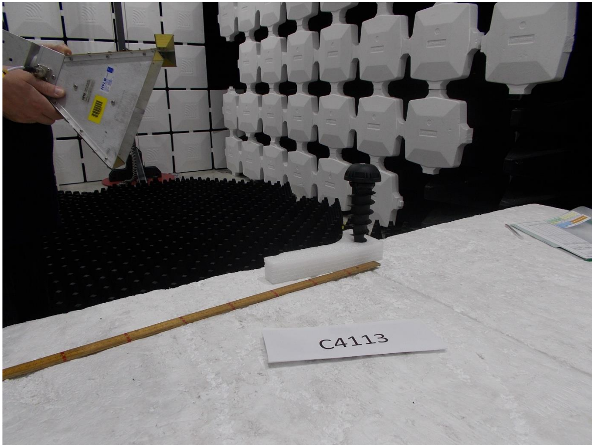
Radiated Emissions 1GHz to 10GHz Exploratory Measurements
