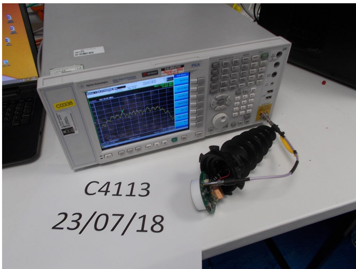
Antenna Port conducted Test (Spectral Density)
