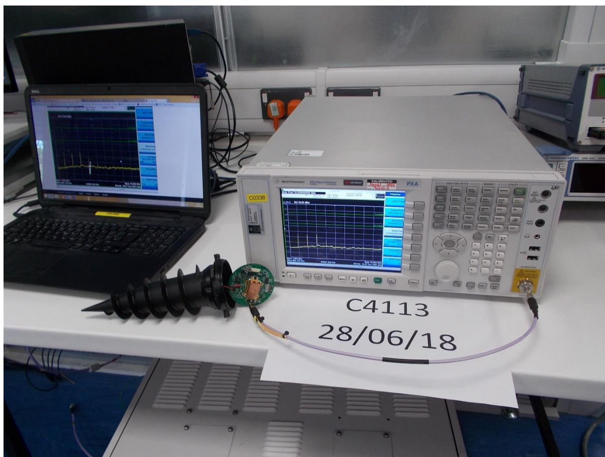
Antenna Port conducted Test (Spurious Emissions)
