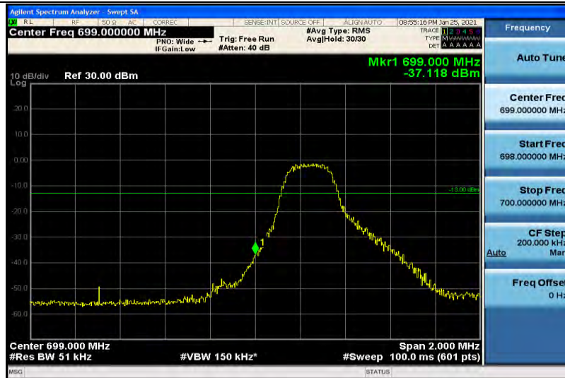
Band12-3MHz-QPSK-23025-1RB#14
