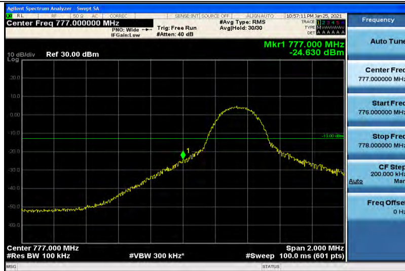
Band13-5MHz-16QAM-23205-1RB#24
