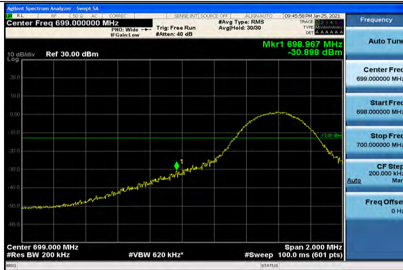
Band12-10MHz-16QAM-23060-1RB#49
