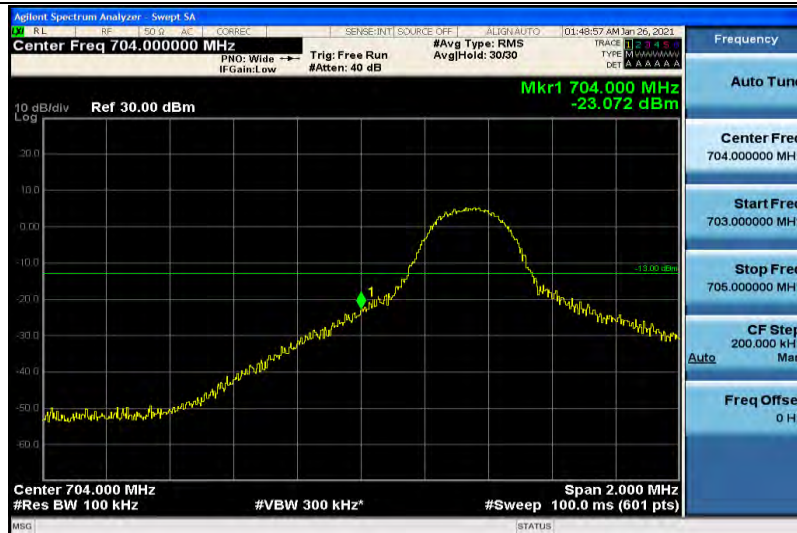
Band17-5MHz-16QAM-23755-1RB#24
