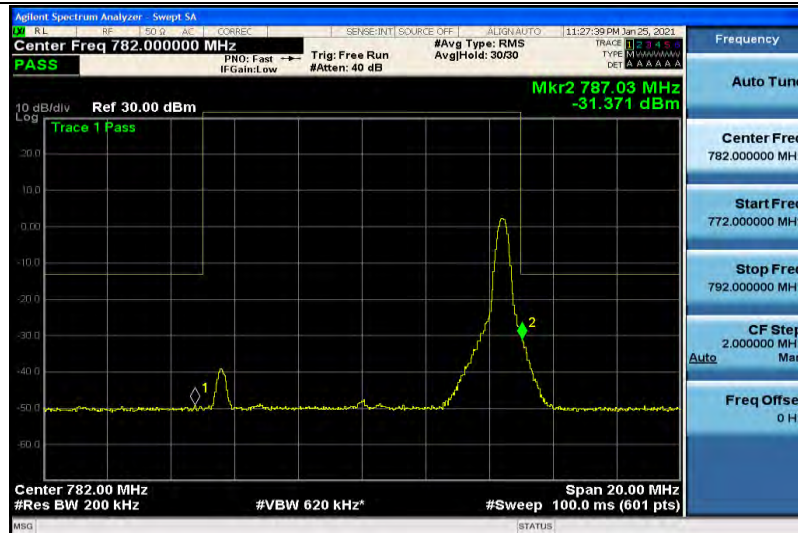
Band13-10MHz-QPSK-23230-1RB#0
