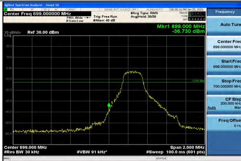
Band12-1.4MHz-QPSK-23017-1RB#5
