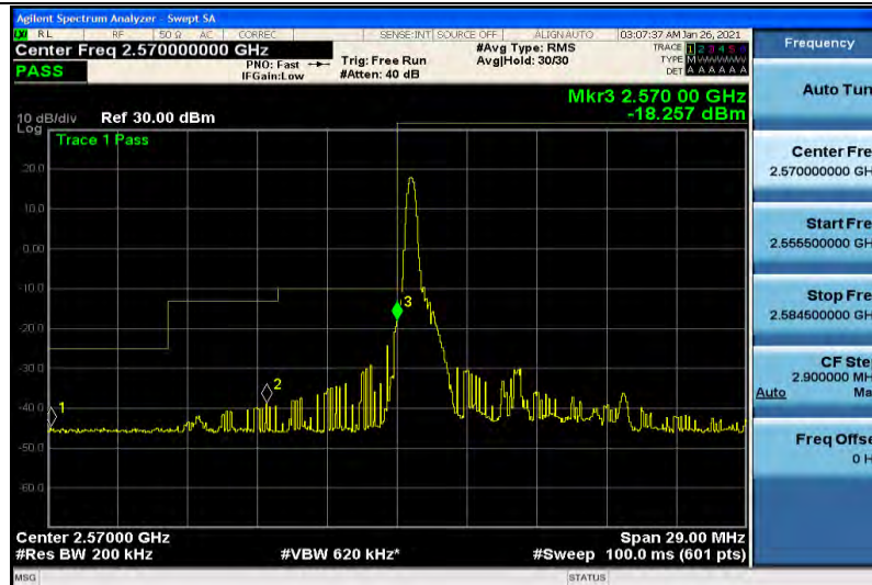
Band38-10MHz-QPSK-37800-1RB#49
