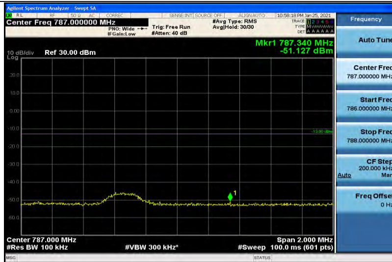
Band13-5MHz-QPSK-23255-1RB#24
