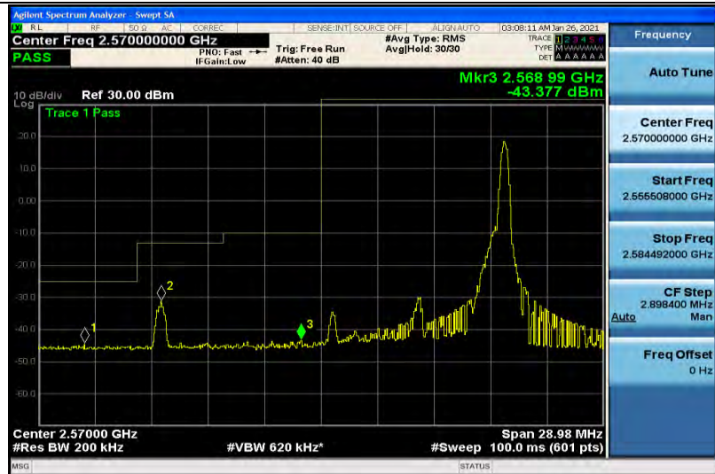
Band38-10MHz-16QAM-37800-1RB#0
