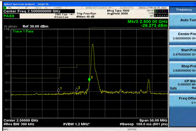
Band7-20MHz-16QAM-20850-1RB#99
