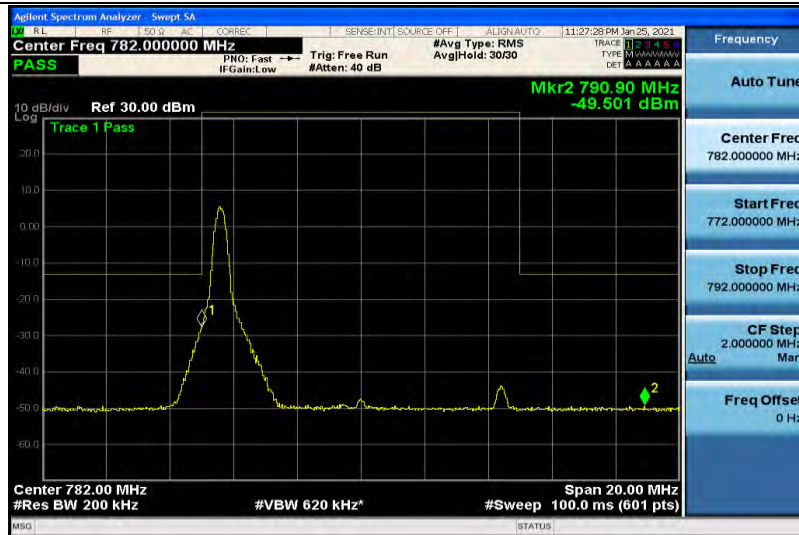
Band13-10MHz-16QAM-23230-1RB#49
