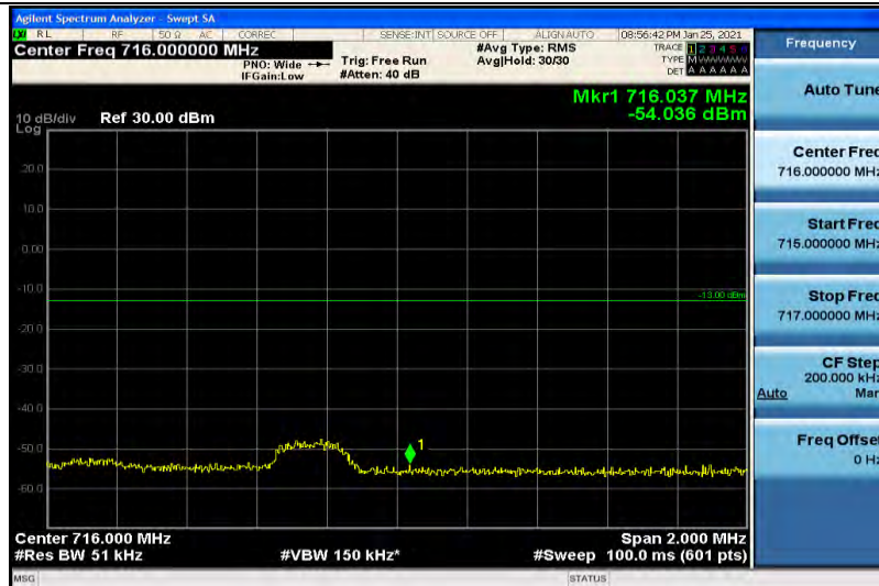
Band12-3MHz-16QAM-23165-1RB#14
