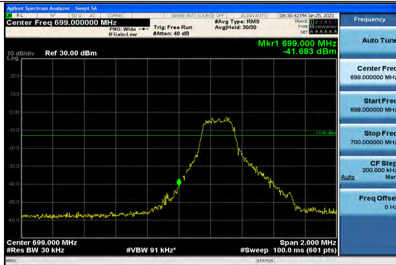
Band12-1.4MHz-16QAM-23017-1RB#5
