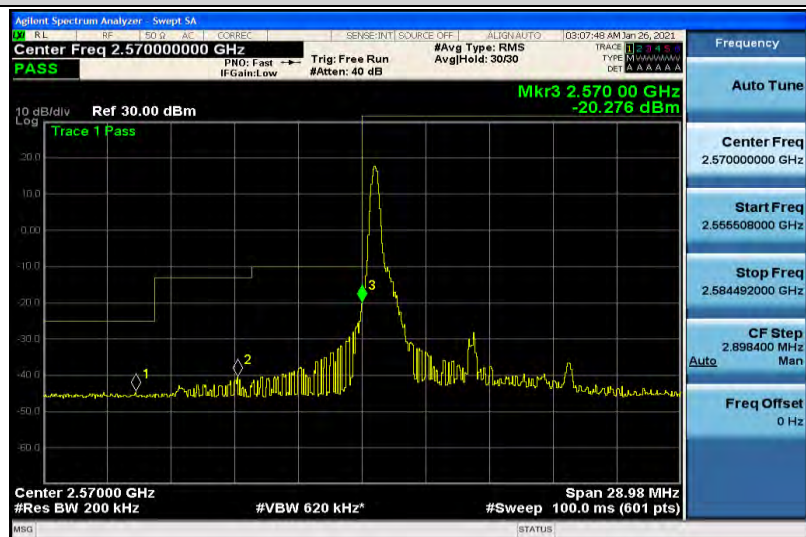
Band38-10MHz-16QAM-37800-50RB#0
