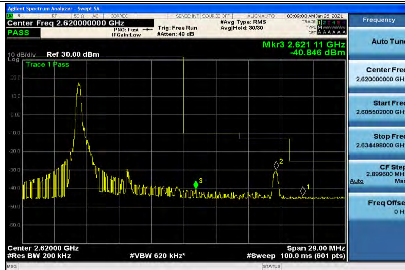
Band38-10MHz-16QAM-38200-1RB#49
