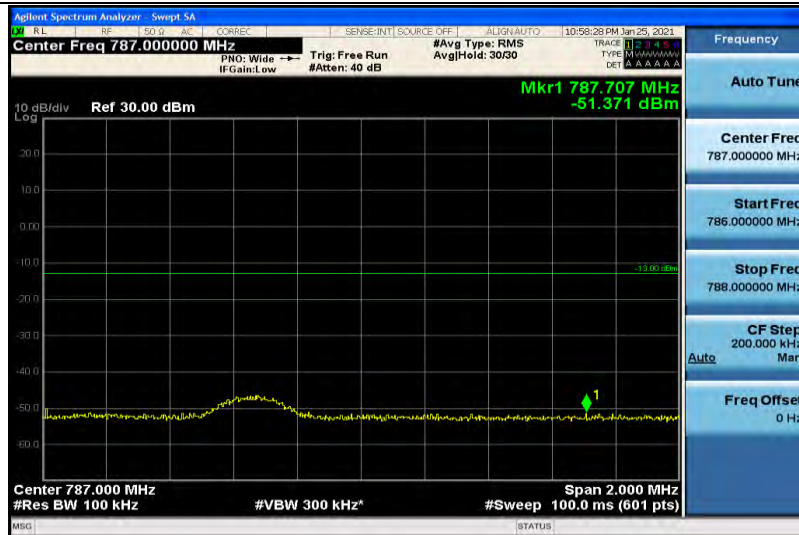
Band13-5MHz-16QAM-23255-1RB#24
