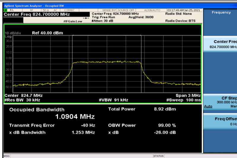
Band5-1.4MHz-QPSK-20525-6RB#0-1.0898
