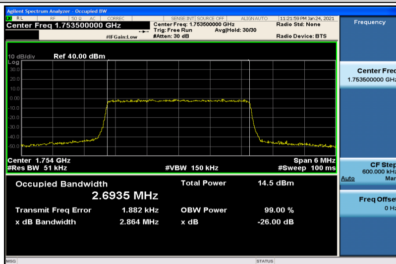
Band4-3MHz-16QAM-19965-15RB#0-2.6878
