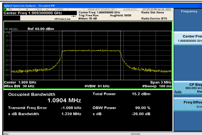
Band2-1.4MHz-QPSK-19193-6RB#0-1.0904
