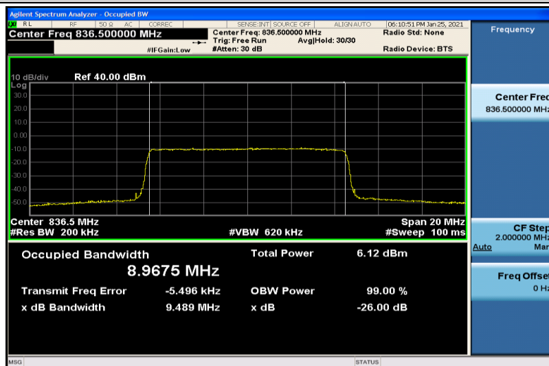
Band5-10MHz-16QAM-20600-50RB#0-8.9966
