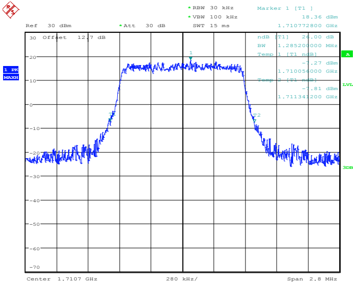
26dB Bandwidth Plot on Channel 19957
