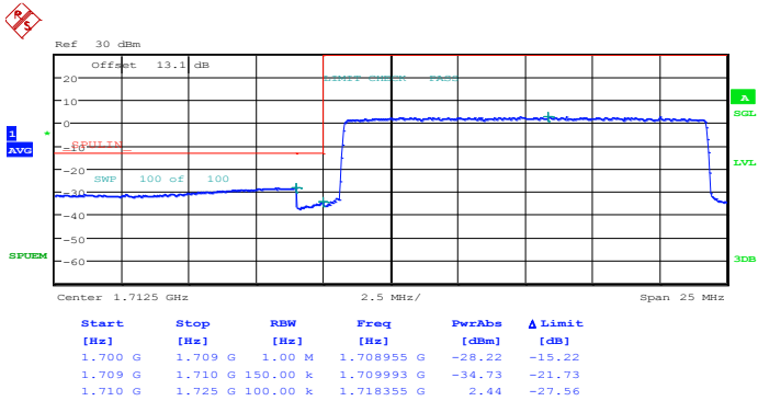
Lower Band Edge Plot for QPSK-RB Size 75, RB Offset 0
