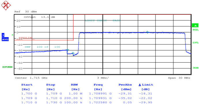
Lower Band Edge Plot for 16QAM-RB Size 100, RB Offset 0
